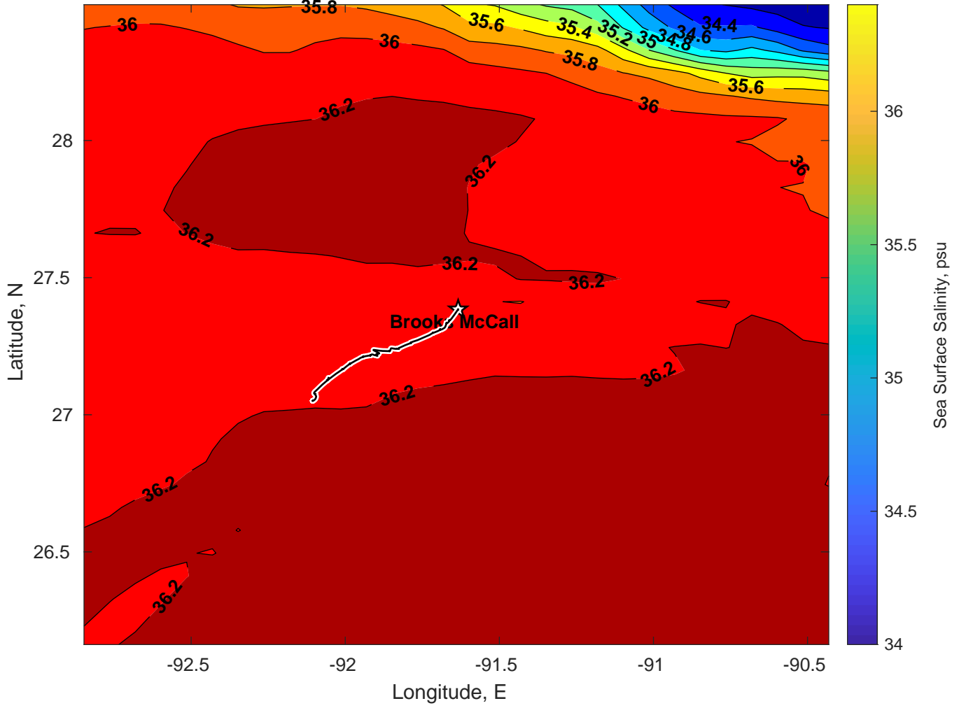
Surface Salinity for Brooks McCall at 01-Apr-2025 00:00:00
