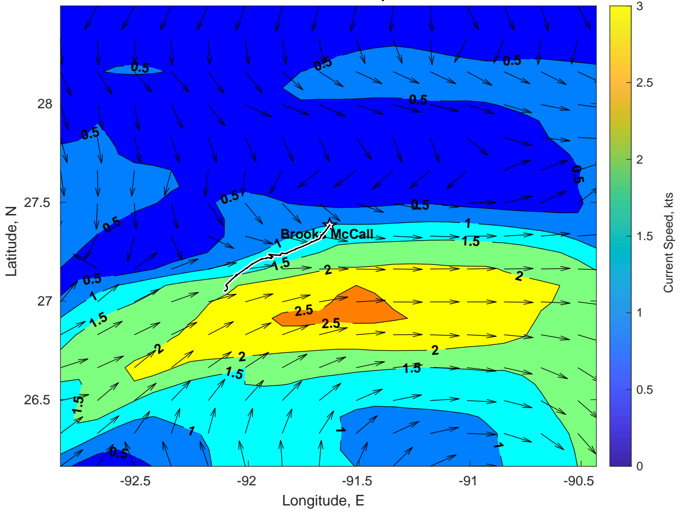
Surface Currents for Brooks McCall at 01-Apr-2025 00:00:00
