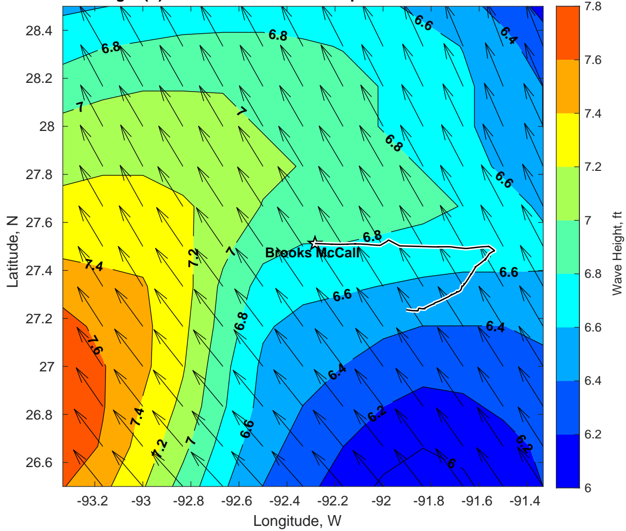
Wave Height (ft) for Brooks McCall at 02-Apr-2025 09:00:00
