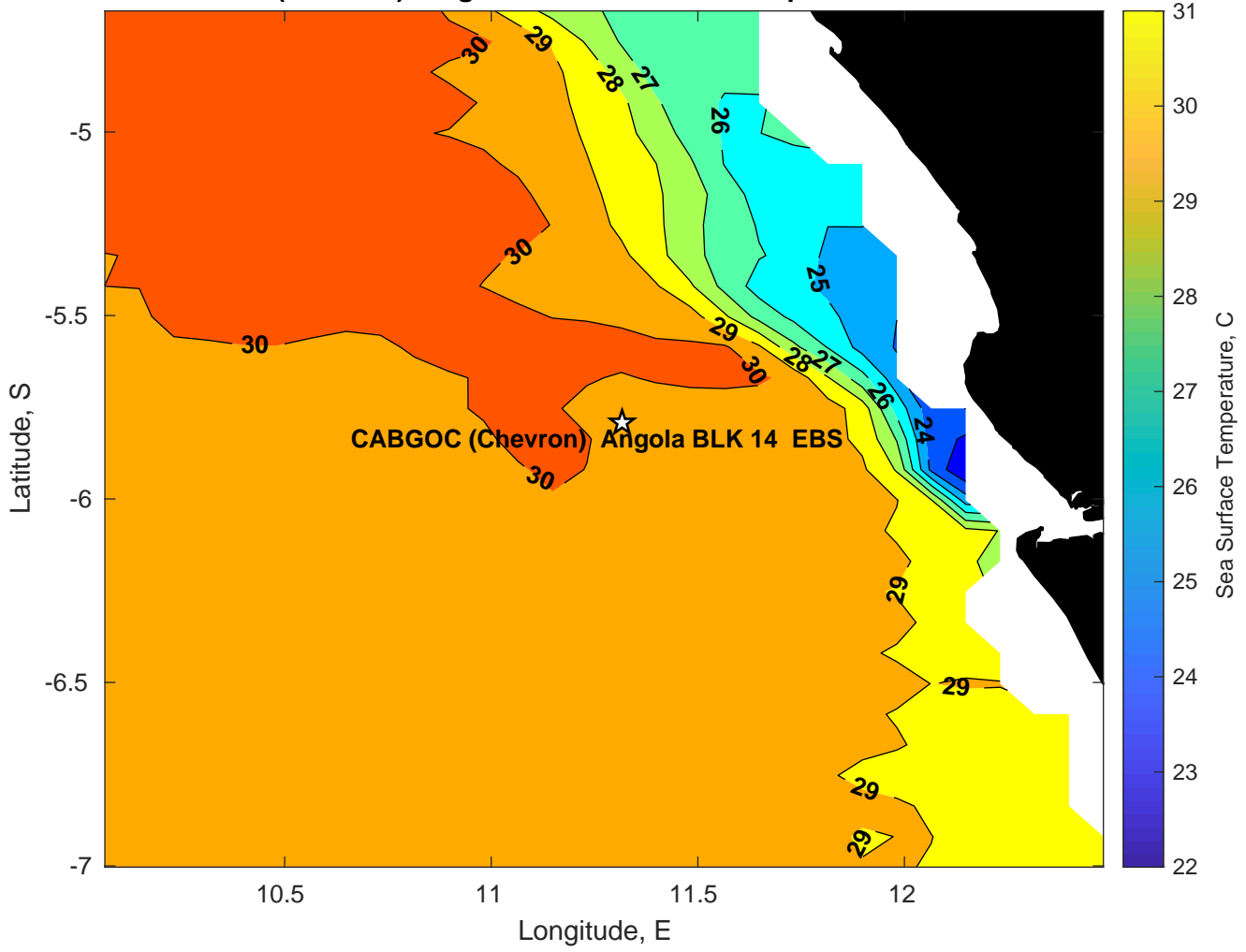
SST for CABGOC (Chevron) Angola BLK 14 EBS at 01-Apr-2025 00:00:00
