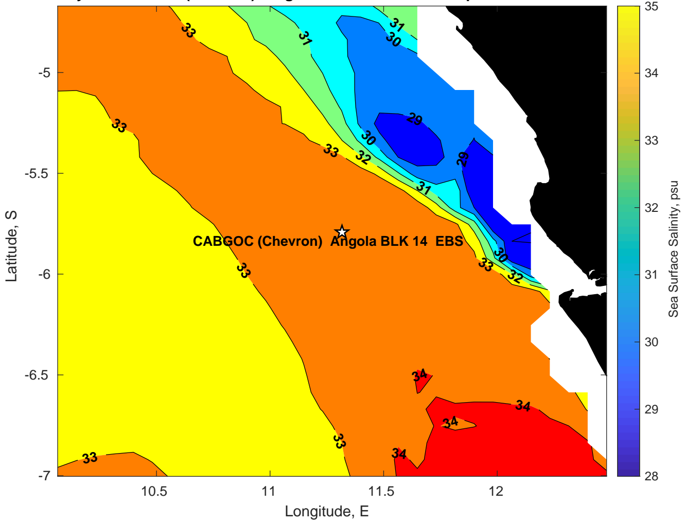
Surface Salinity for CABGOC (Chevron) Angola BLK 14 EBS at 01-Apr-2025 00:00:00
