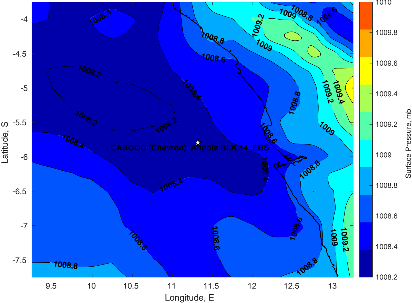
Surface Pressure (mb) for CABGOC (Chevron) Angola BLK 14 EBS at 03-Apr-2025 00:00:00
