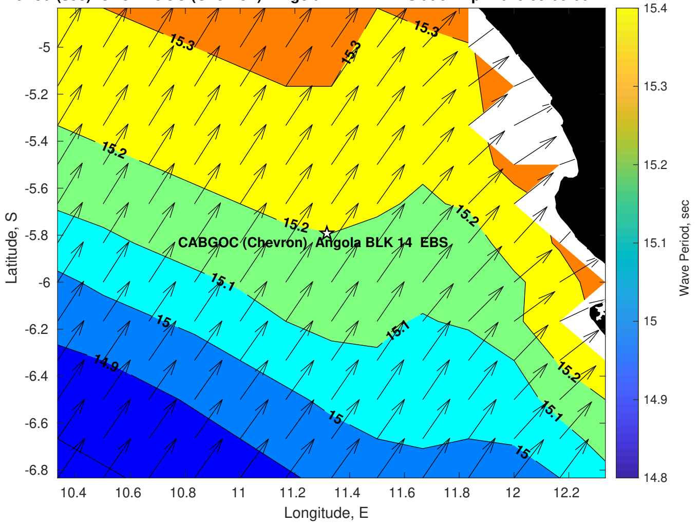
Wave Period (sec) for CABGOC (Chevron) Angola BLK 14 EBS at 02-Apr-2025 09:00:00
