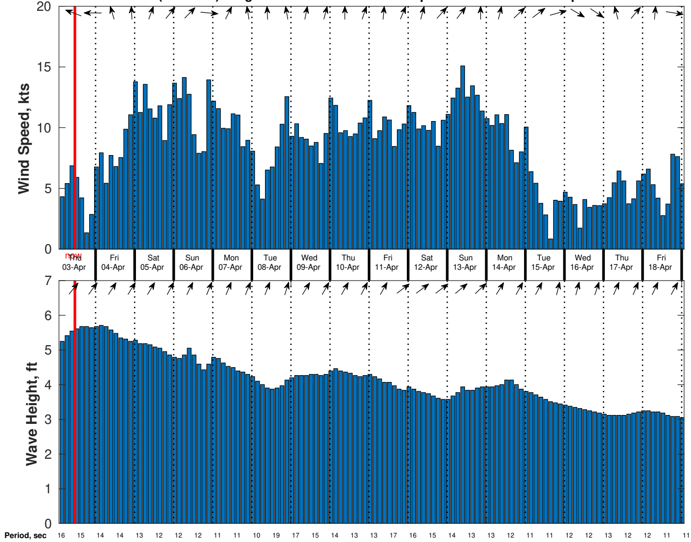
Wind & Wave Forecast for CABGOC (Chevron) Angola BLK 14 EBS from 02-Apr-2025 02:00:00 to 18-Apr-2025 02:00:00
