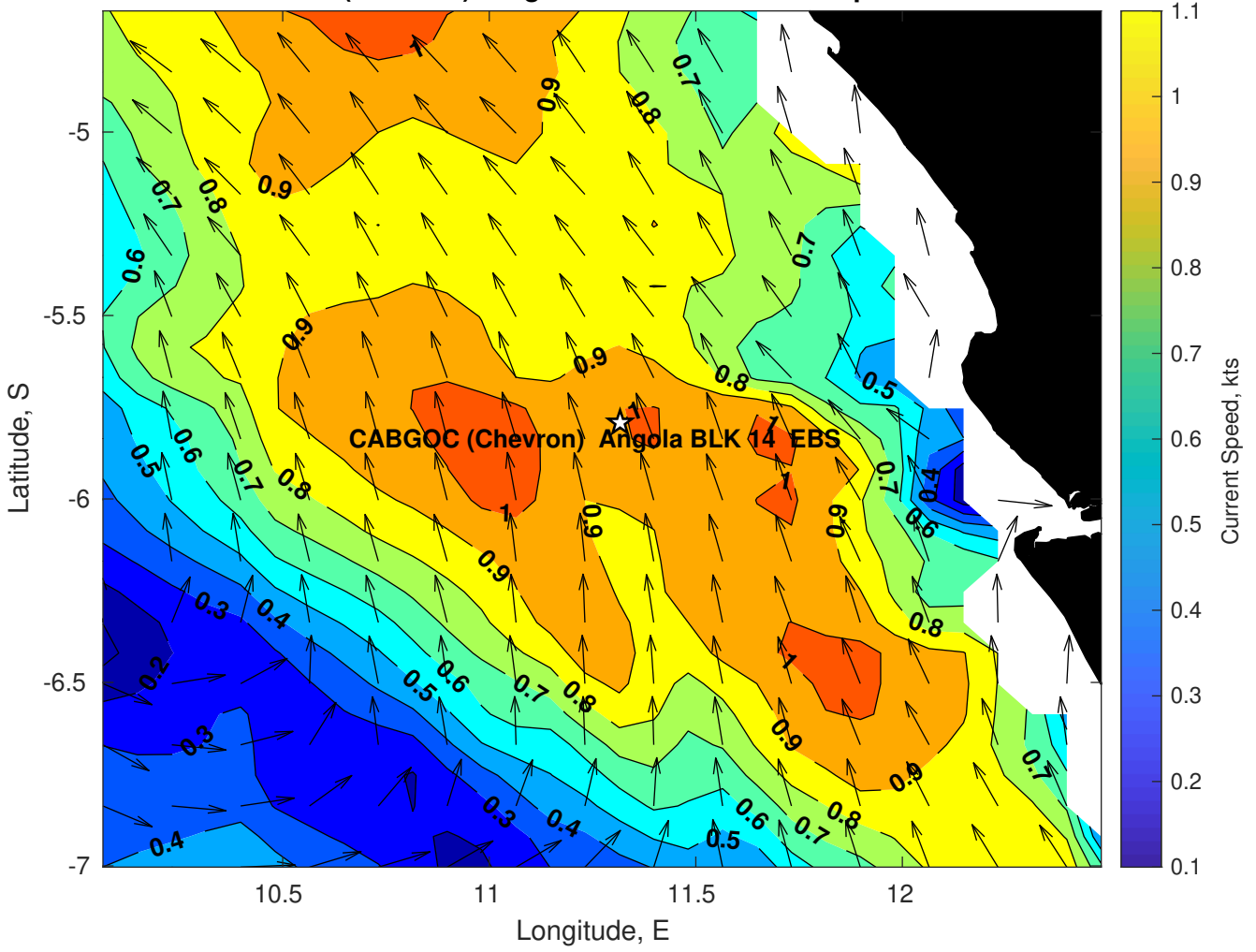
Surface Currents for CABGOC (Chevron) Angola BLK 14 EBS at 01-Apr-2025 00:00:00
