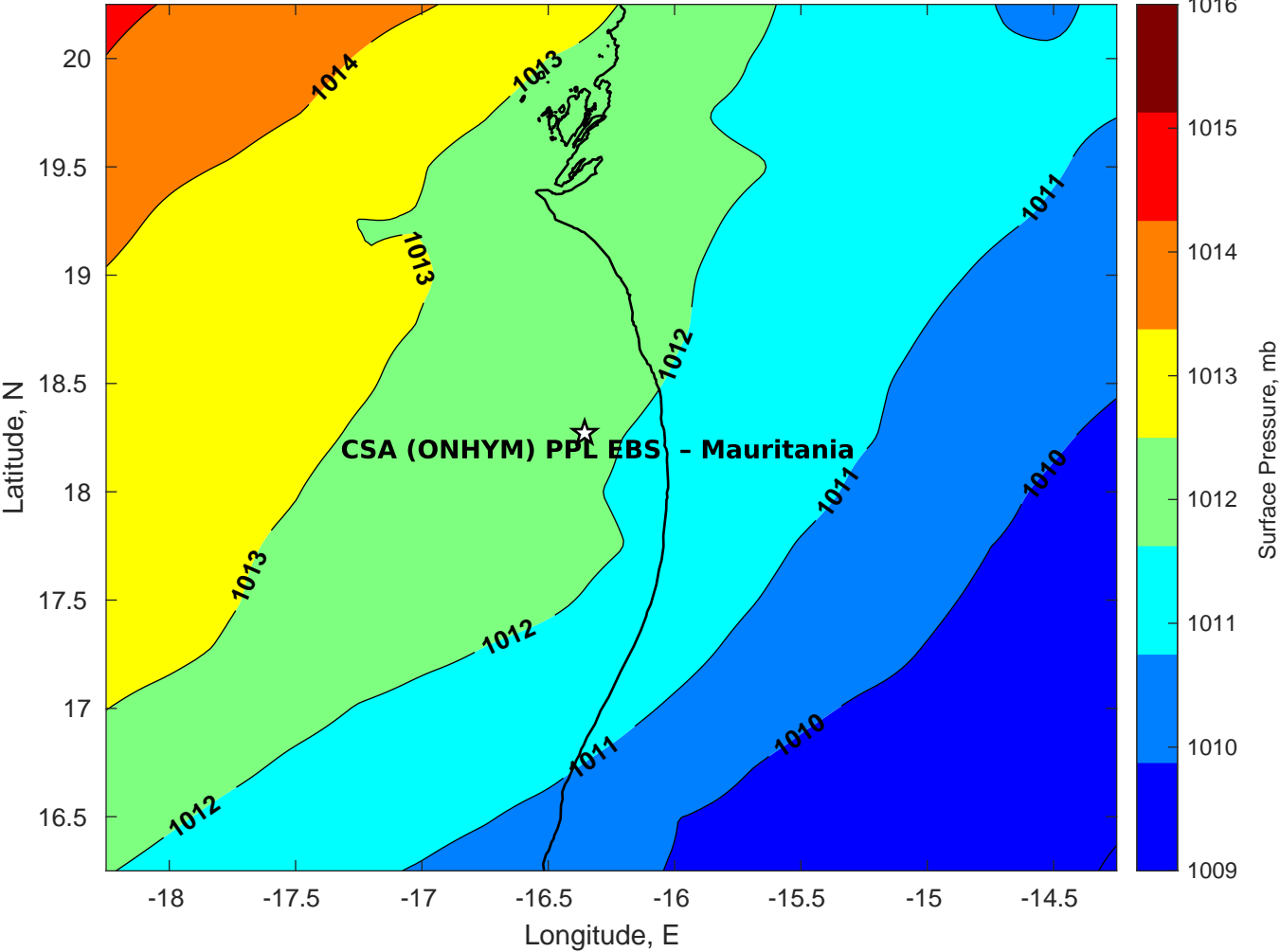
Surface Pressure (mb) for CSA (ONHYM) PPL EBS - Mauritania at 02-Apr-2025 00:00:00
