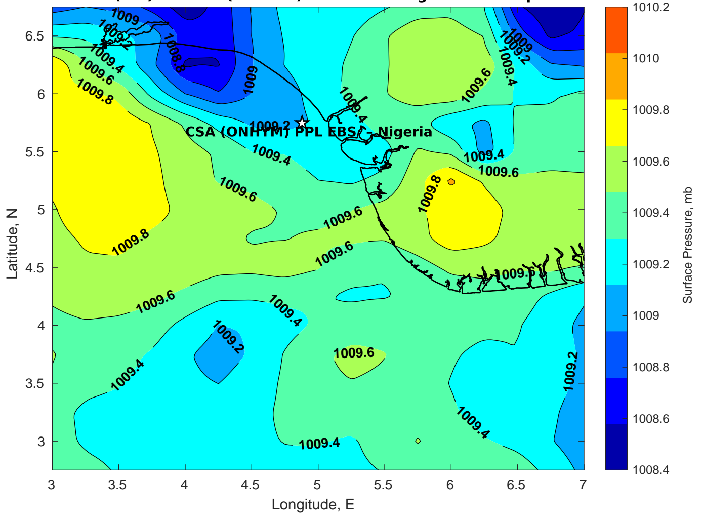
Surface Pressure (mb) for CSA (ONHYM) PPL EBS - Nigeria at 03-Apr-2025 00:00:00
