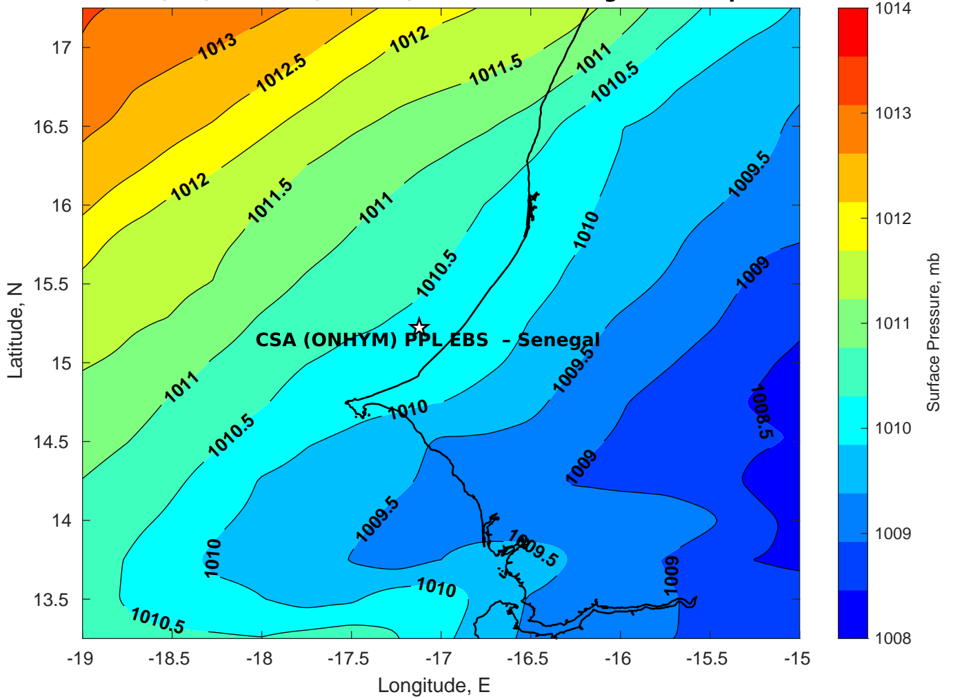
Surface Pressure (mb) for CSA (ONHYM) PPL EBS - Senegal at 02-Apr-2025 00:00:00
