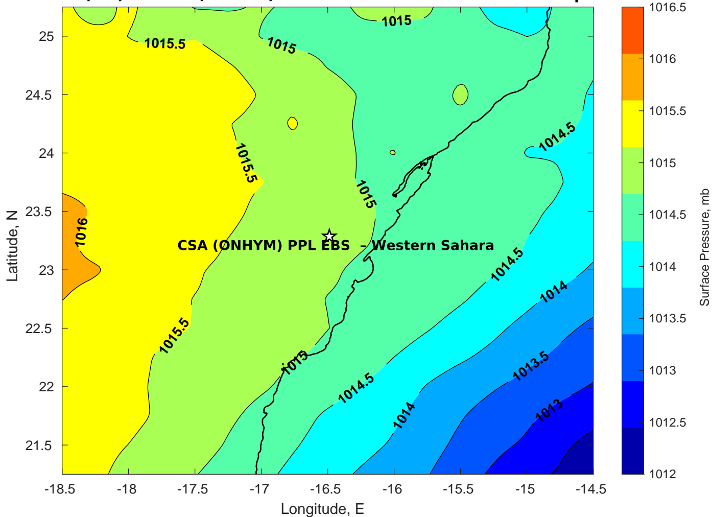
Surface Pressure (mb) for CSA (ONHYM) PPL EBS - Western Sahara at 02-Apr-2025 00:00:00
