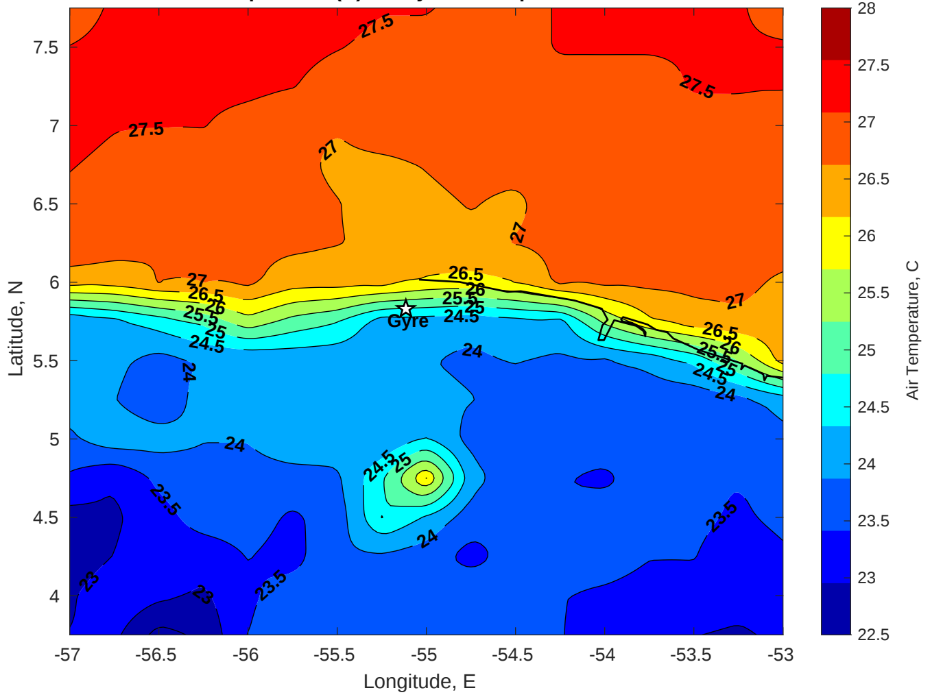
Air Temperature (C) for Gyre at 02-Apr-2025
