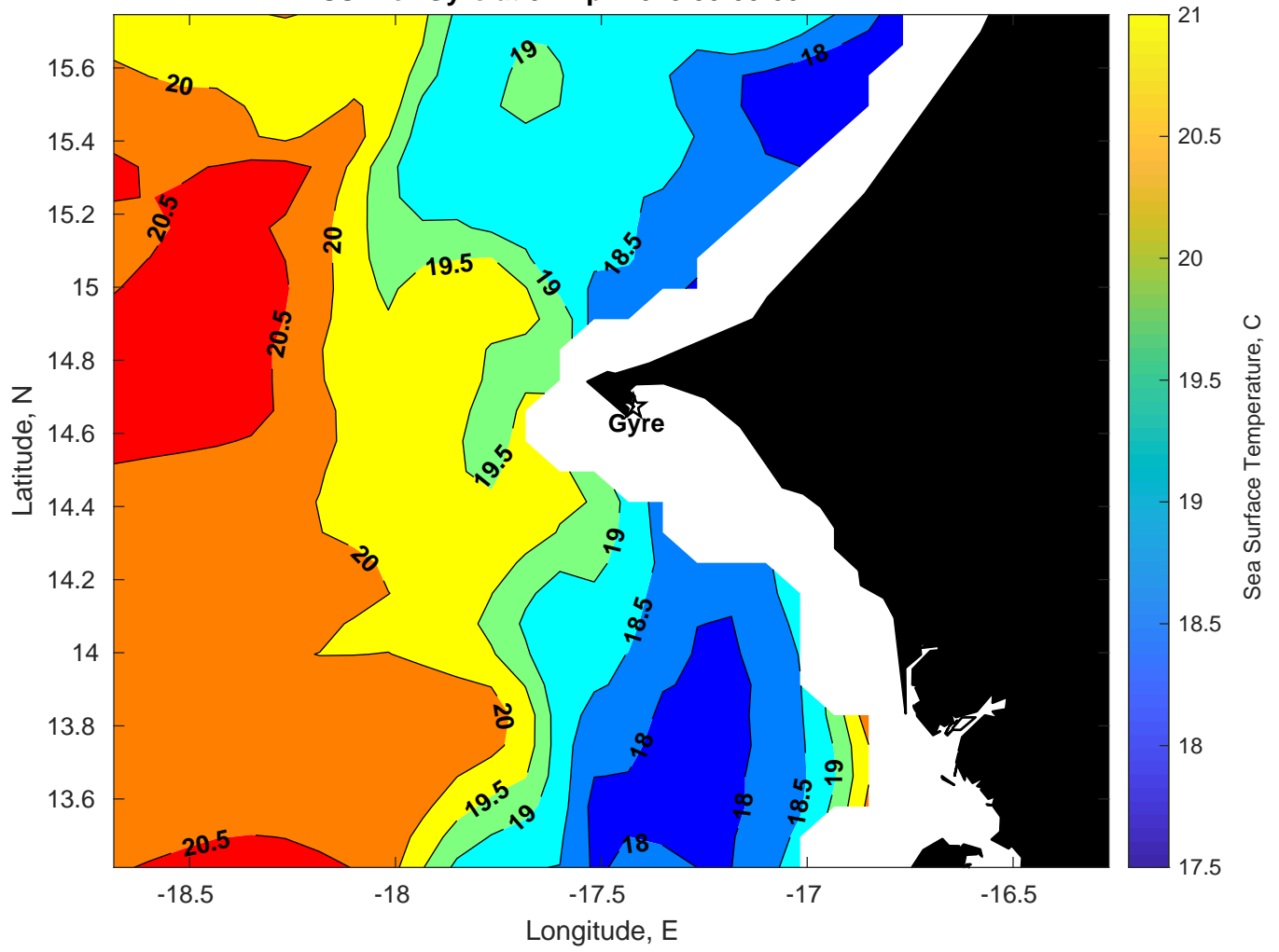
SST for Gyre at 01-Apr-2025 00:00:00
