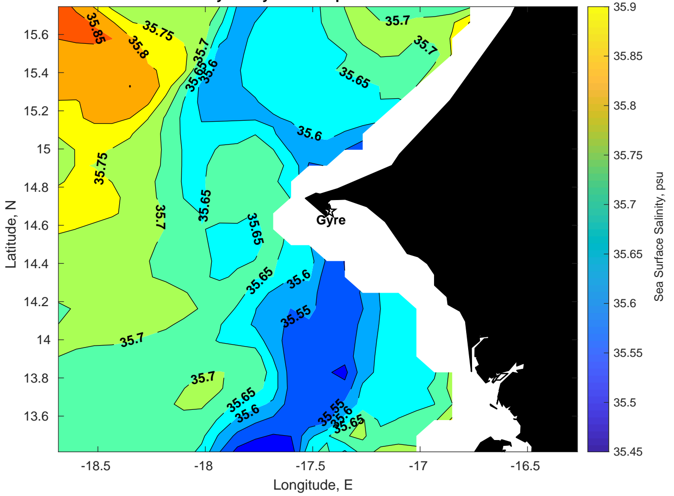
Surface Salinity for Gyre at 01-Apr-2025 00:00:00
