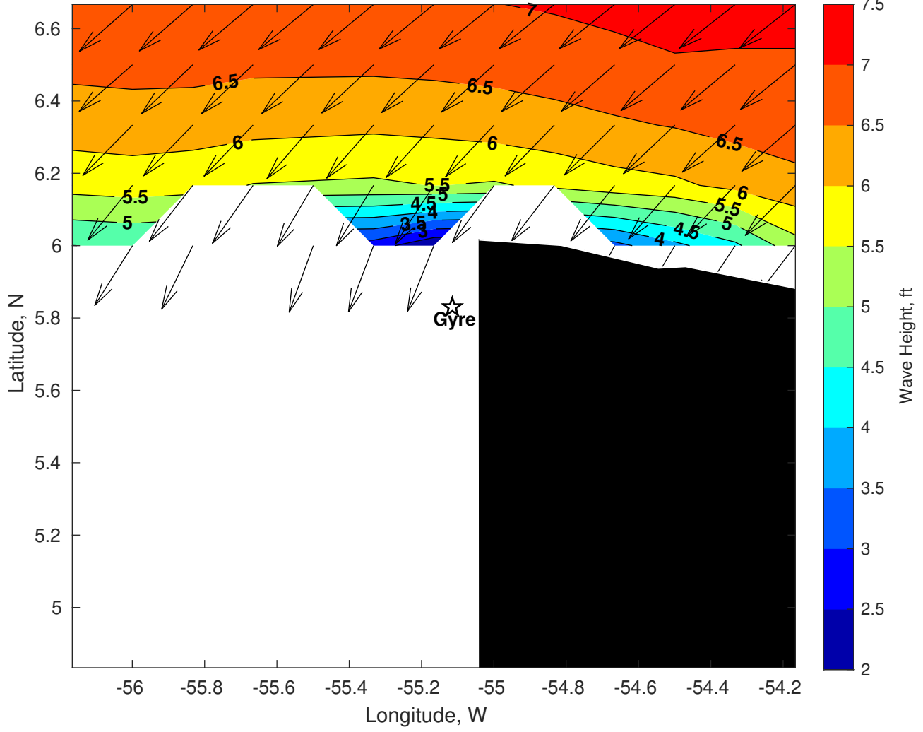
Wave Height (ft) for Gyre at 02-Apr-2025 09:00:00
