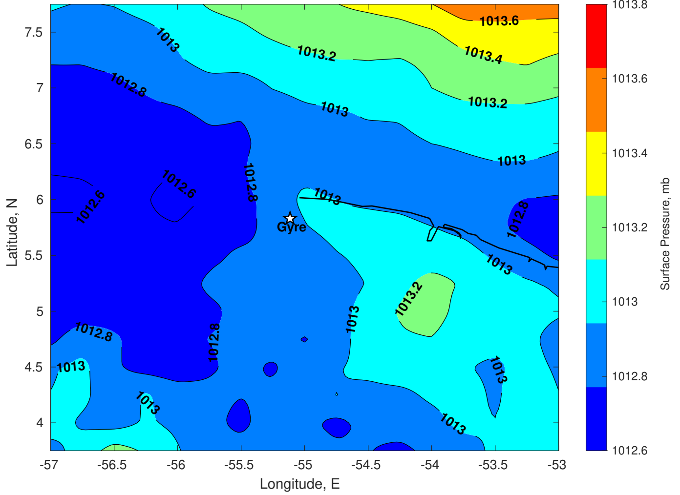
Surface Pressure (mb) for Gyre at 02-Apr-2025 00:00:00
