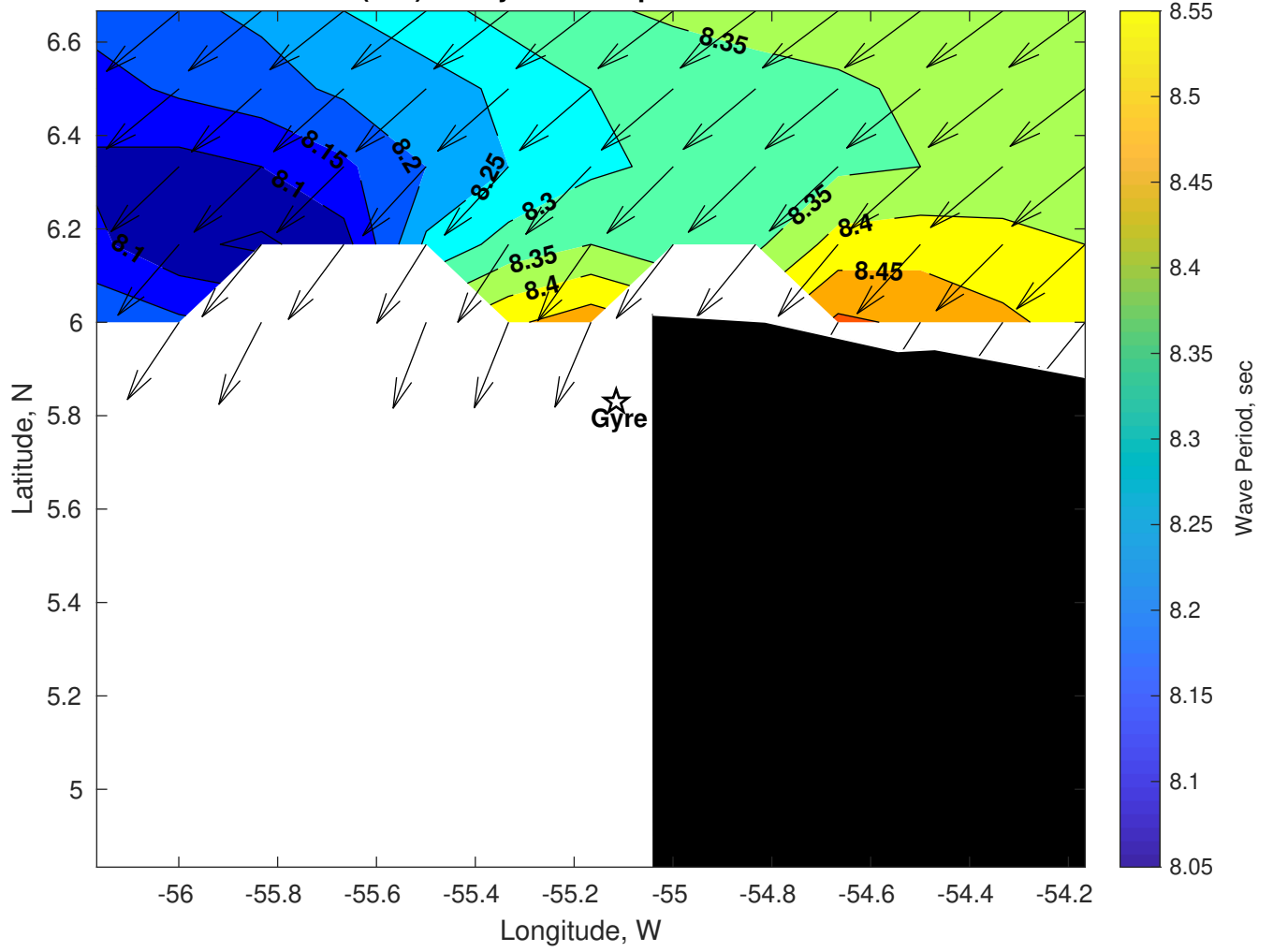
Wave Period (sec) for Gyre at 02-Apr-2025 09:00:00
