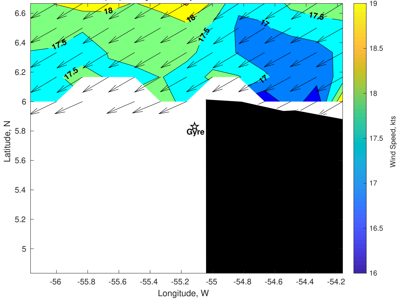
Winds (kts) for Gyre at 02-Apr-2025 09:00:00
