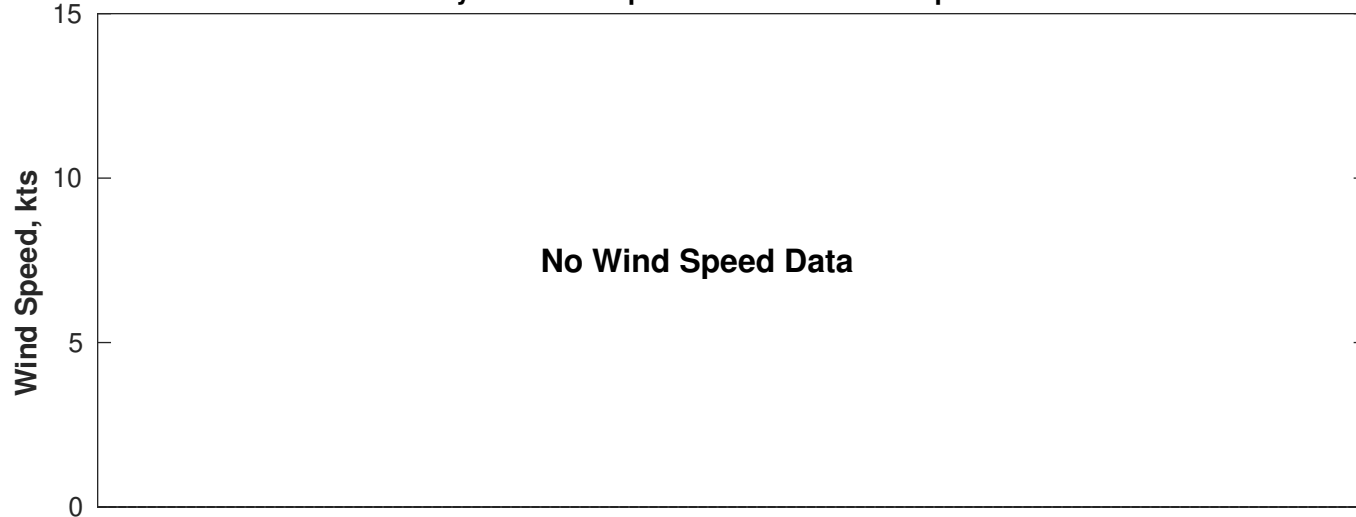
Wind & Wave Forecast for Gyre from 01-Apr-2025 20:00:00 to 17-Apr-2025 20:00:00
