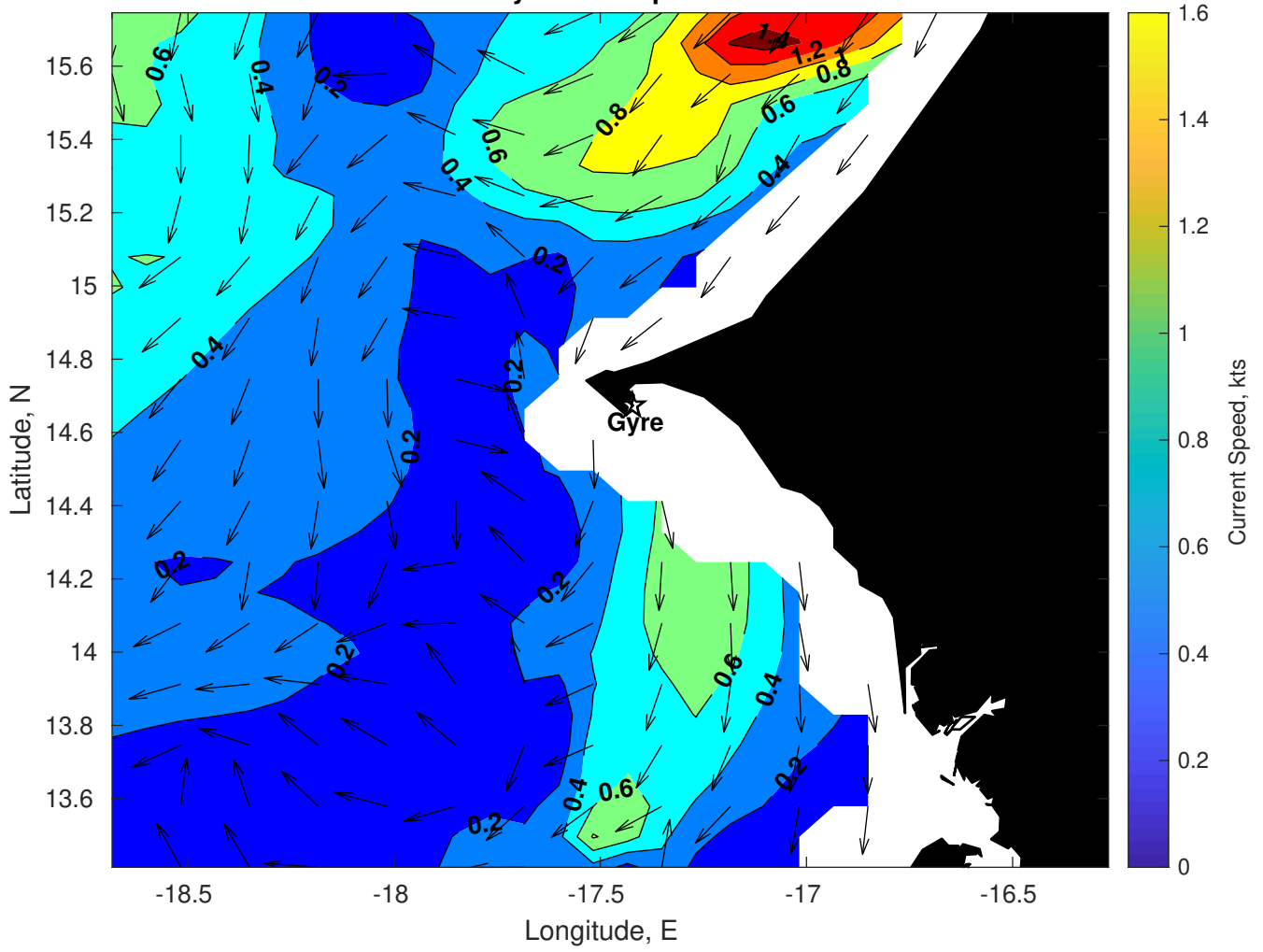
Surface Currents for Gyre at 01-Apr-2025 00:00:00
