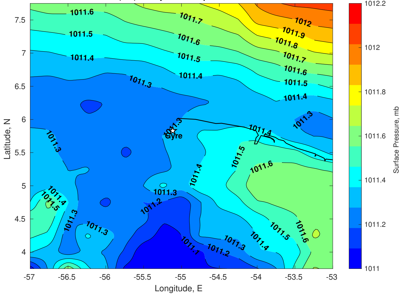
Surface Pressure (mb) for Gyre at 03-Apr-2025 00:00:00
