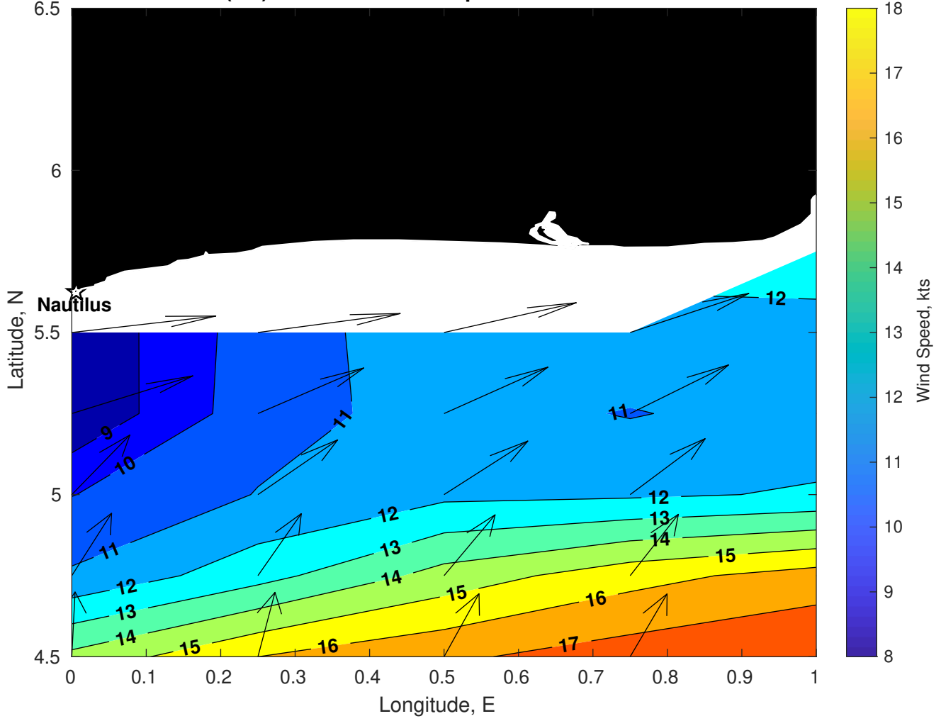
Winds (kts) for Nautilus at 02-Apr-2025 09:00:00
