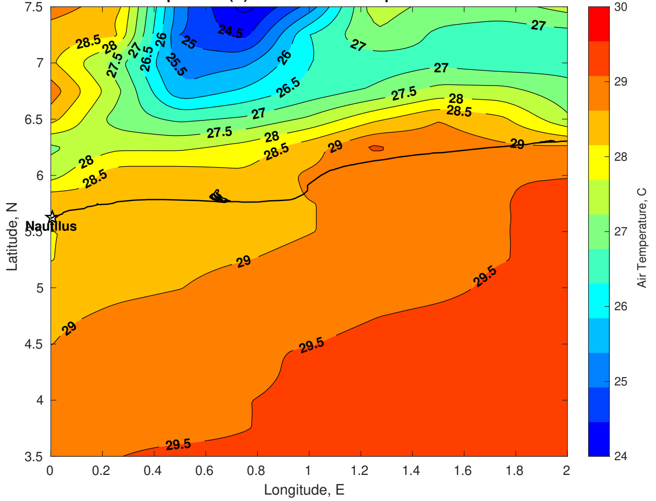
Air Temperature (C) for Nautilus at 02-Apr-2025
