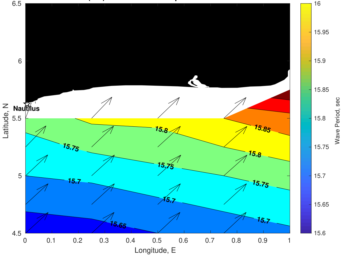
Wave Period (sec) for Nautilus at 02-Apr-2025 09:00:00
