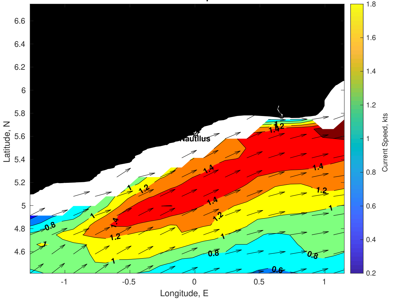
Surface Currents for Nautilus at 01-Apr-2025 00:00:00
