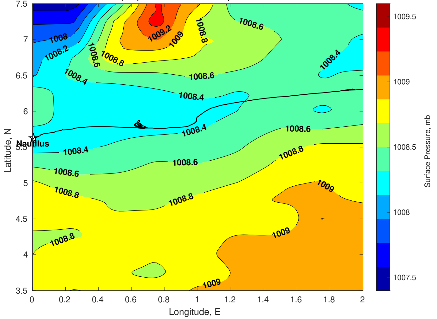
Surface Pressure (mb) for Nautilus at 02-Apr-2025 00:00:00
