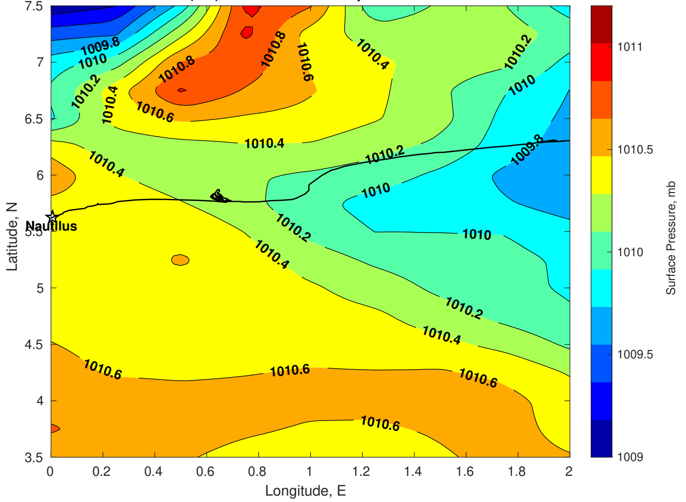
Surface Pressure (mb) for Nautilus at 04-Apr-2025 00:00:00
