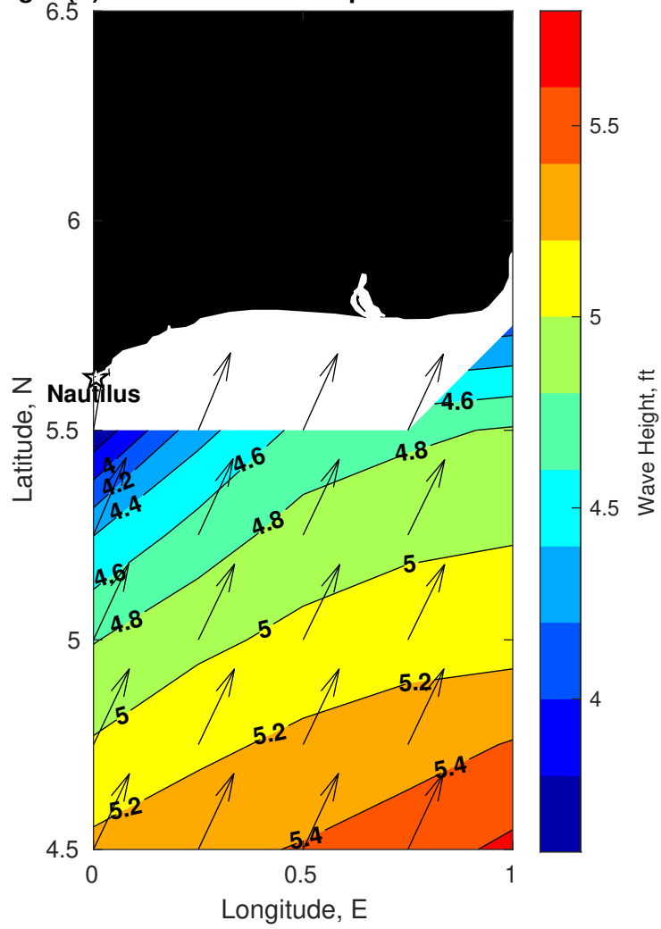
Wave Height (ft) for Nautilus at 02-Apr-2025 09:00:00
