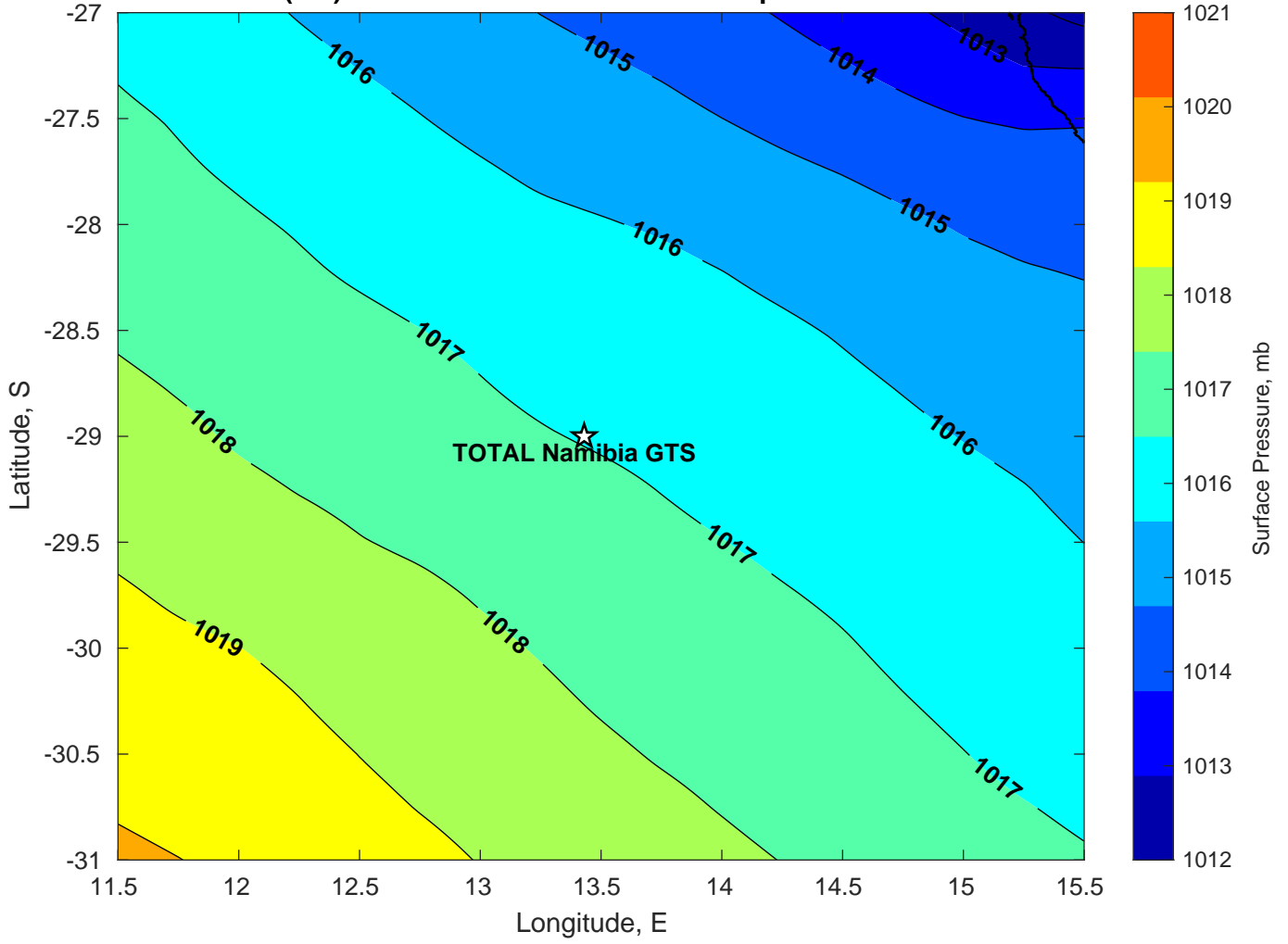
Surface Pressure (mb) for TOTAL Namibia GTS at 02-Apr-2025 00:00:00
