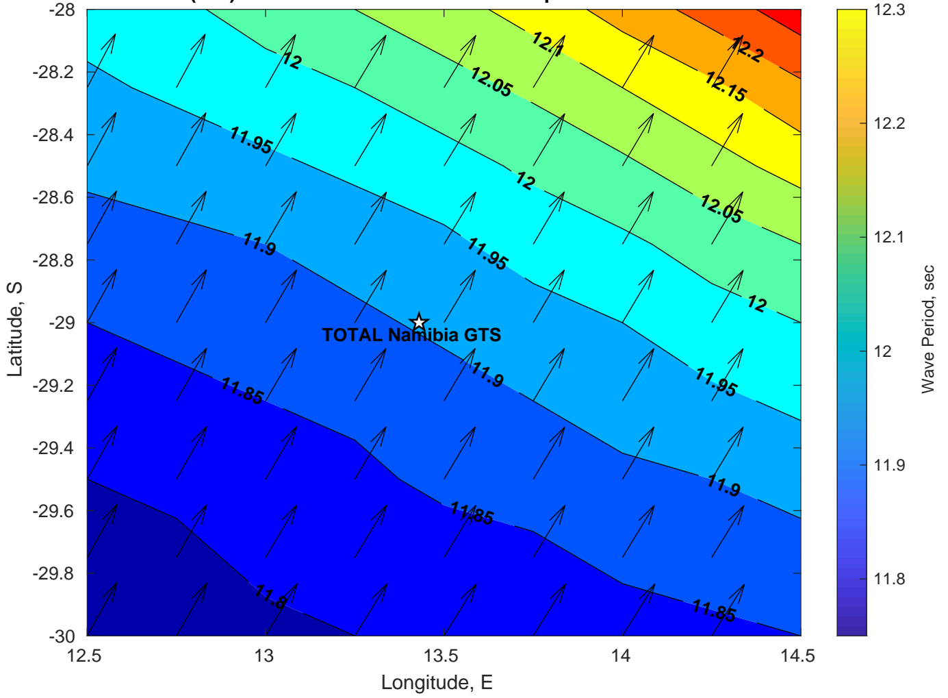
Wave Period (sec) for TOTAL Namibia GTS at 02-Apr-2025 09:00:00
