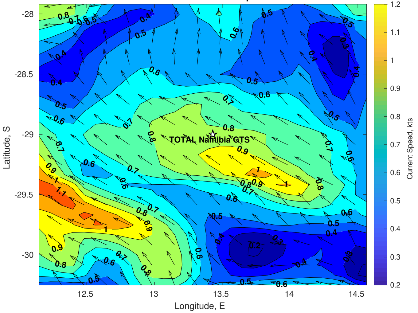
Surface Currents for TOTAL Namibia GTS at 01-Apr-2025 00:00:00
