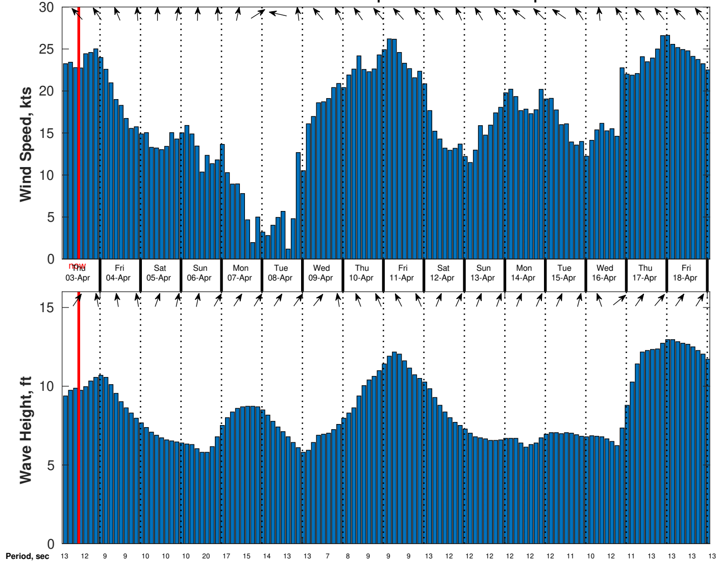
Wind & Wave Forecast for TOTAL Namibia GTS from 02-Apr-2025 02:00:00 to 18-Apr-2025 02:00:00
