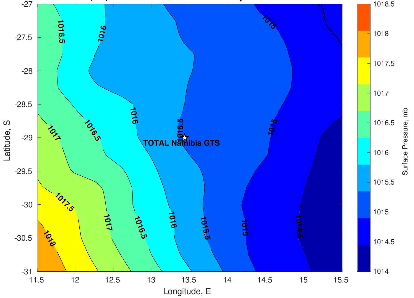
Surface Pressure (mb) for TOTAL Namibia GTS at 04-Apr-2025 00:00:00
