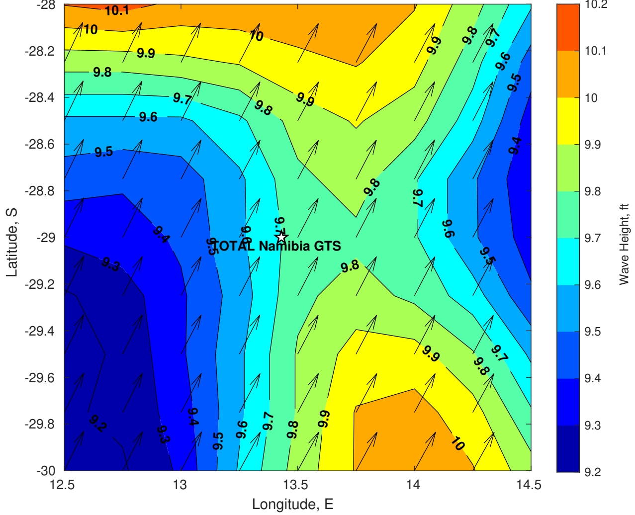
Wave Height (ft) for TOTAL Namibia GTS at 02-Apr-2025 09:00:00
