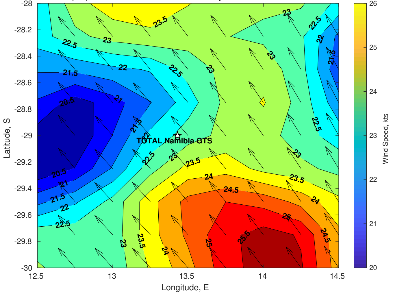
Winds (kts) for TOTAL Namibia GTS at 02-Apr-2025 09:00:00
