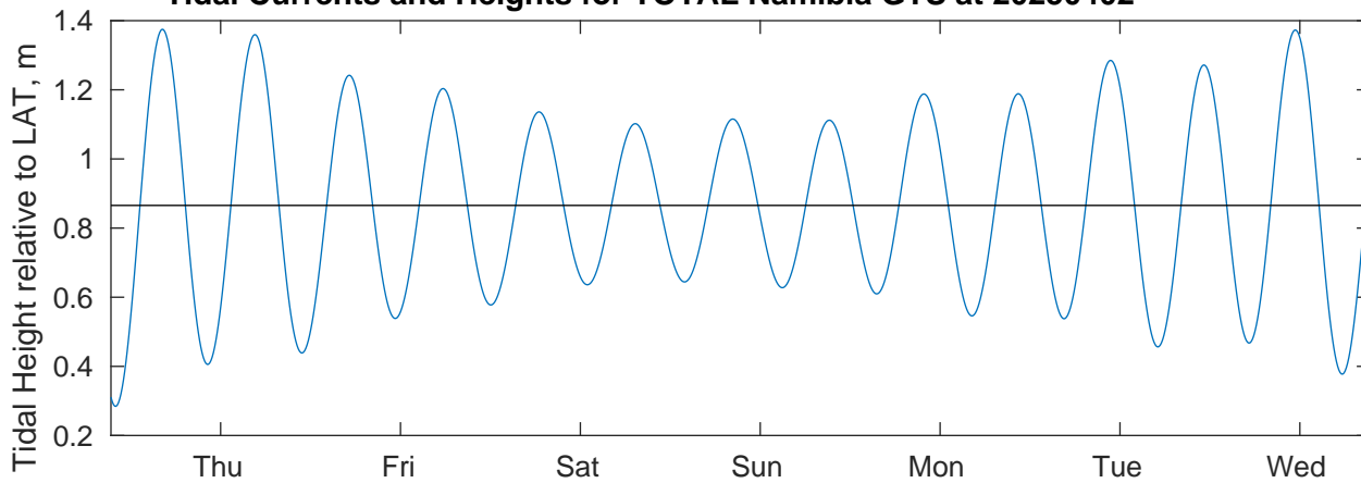
Tidal Currents and Heights for TOTAL Namibia GTS at 20250402
