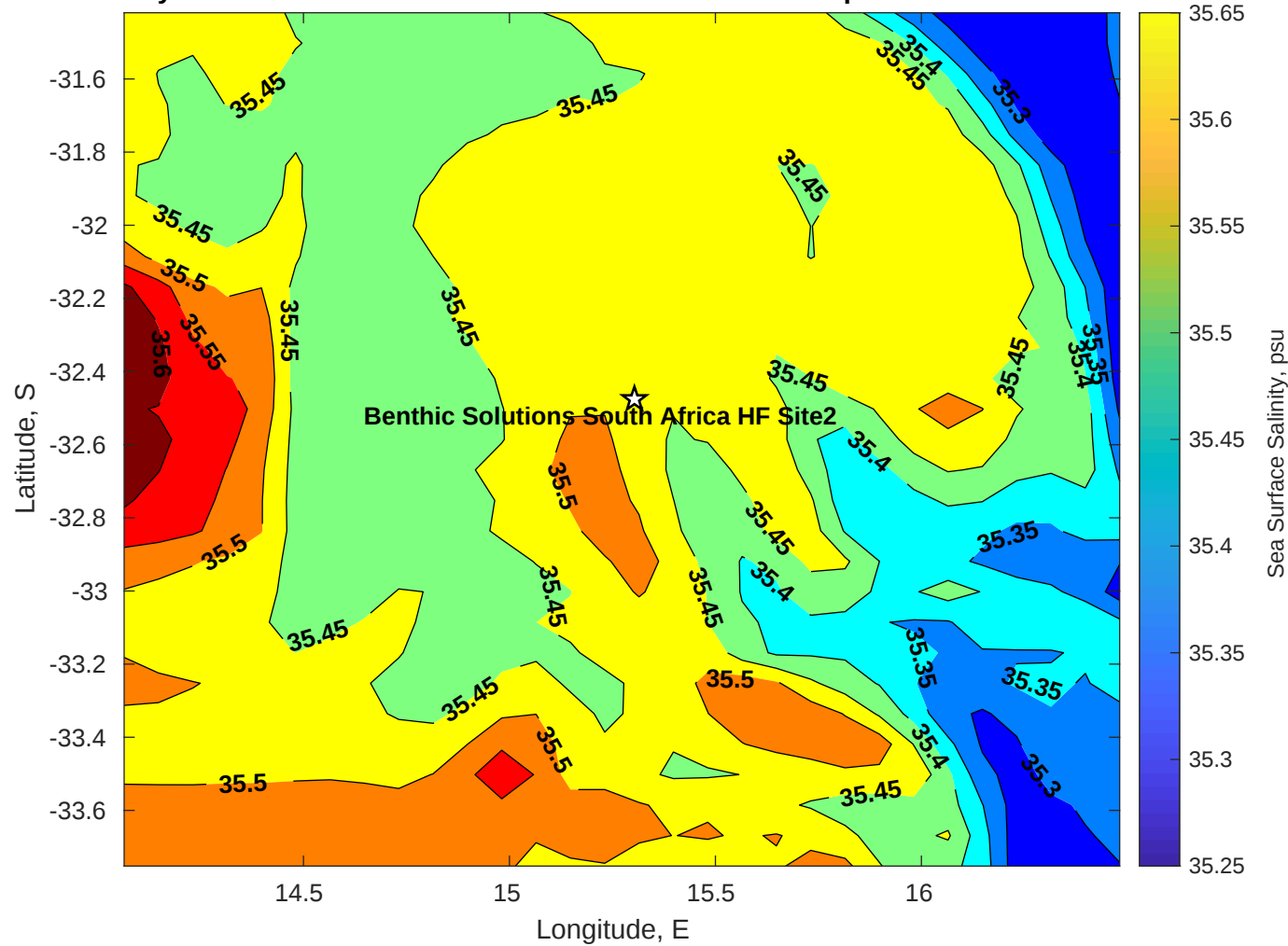
Surface Salinity for Benthic Solutions South Africa HF Site2 at 02-Apr-2025 00:00:00
