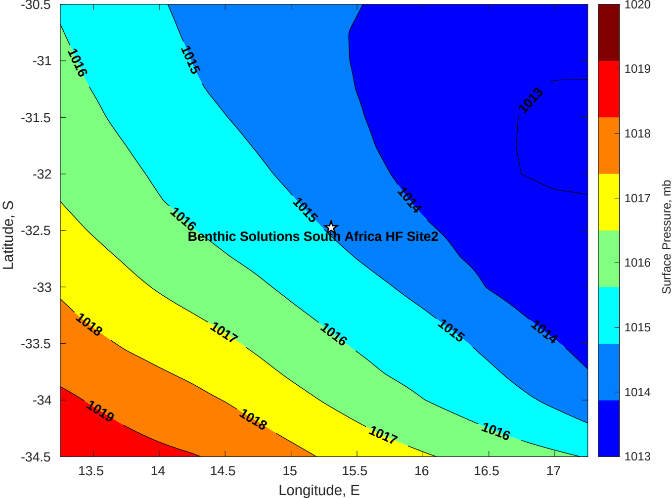
Surface Pressure (mb) for Benthic Solutions South Africa HF Site2 at 04-Apr-2025 00:00:00
