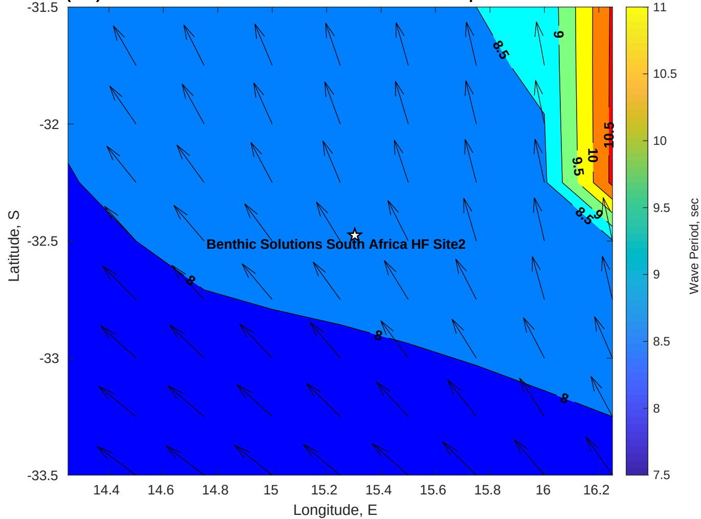
Wave Period (sec) for Benthic Solutions South Africa HF Site2 at 03-Apr-2025 09:00:00
