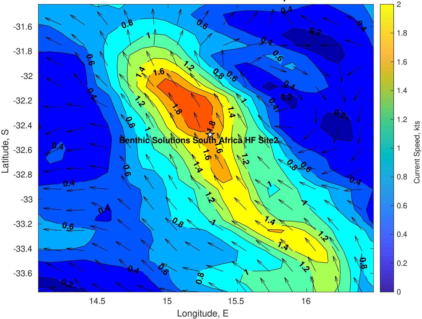
Surface Currents for Benthic Solutions South Africa HF Site2 at 02-Apr-2025 00:00:00
