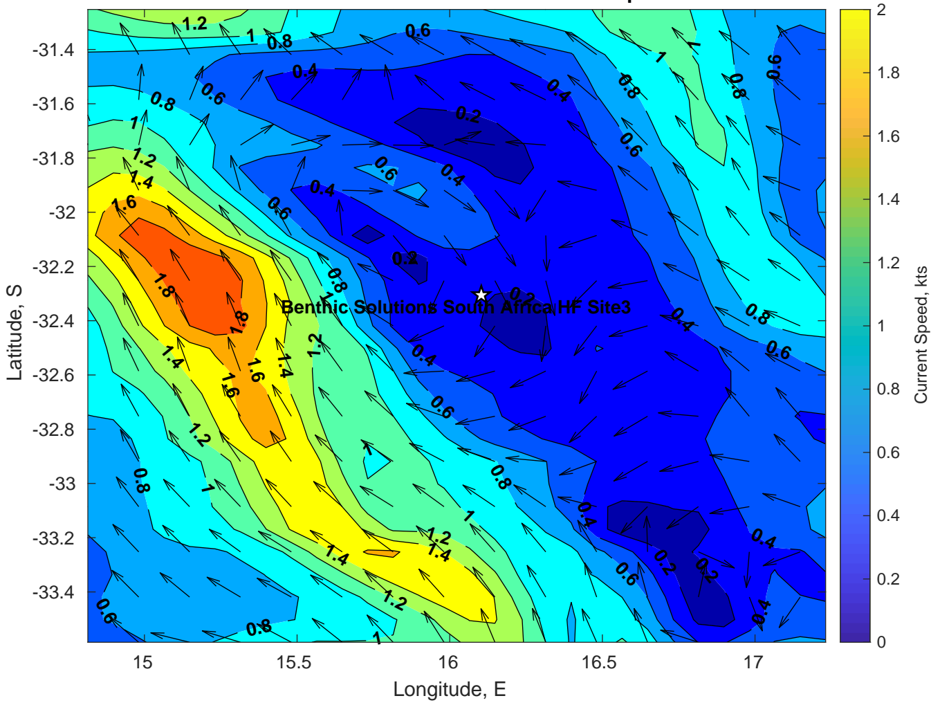
Surface Currents for Benthic Solutions South Africa HF Site3 at 02-Apr-2025 00:00:00
