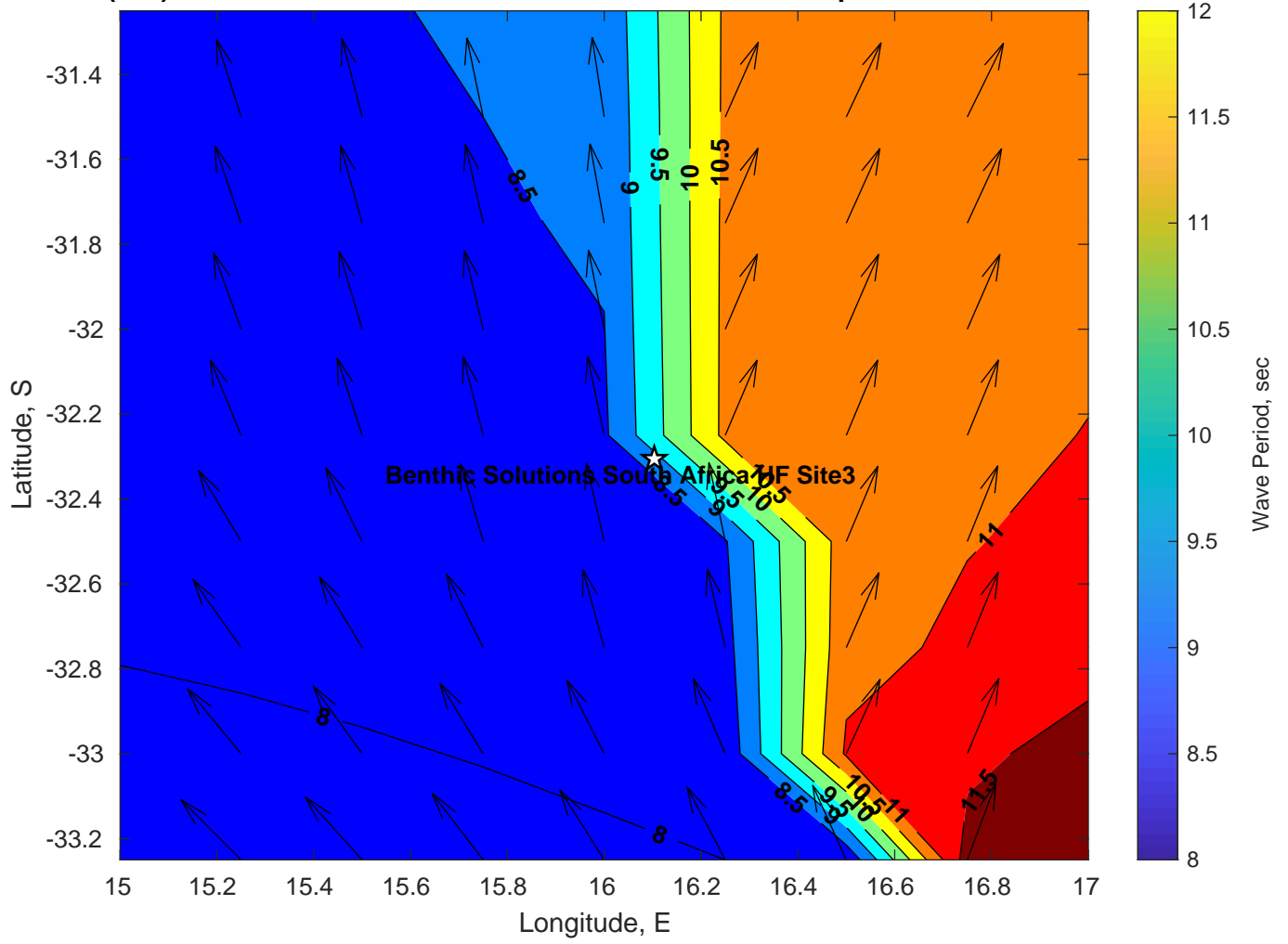
Wave Period (sec) for Benthic Solutions South Africa HF Site3 at 03-Apr-2025 09:00:00
