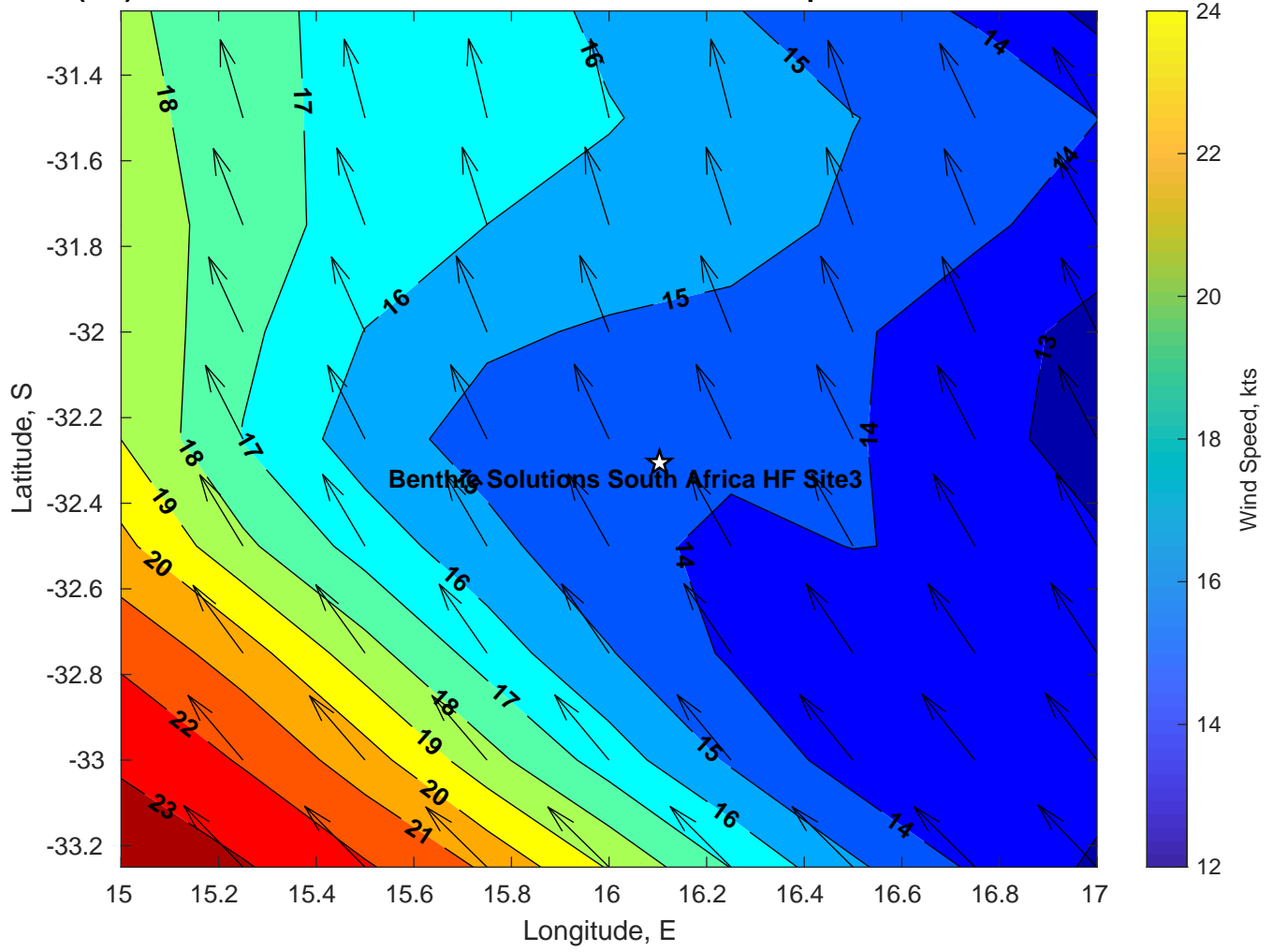
Winds (kts) for Benthic Solutions South Africa HF Site3 at 03-Apr-2025 09:00:00
