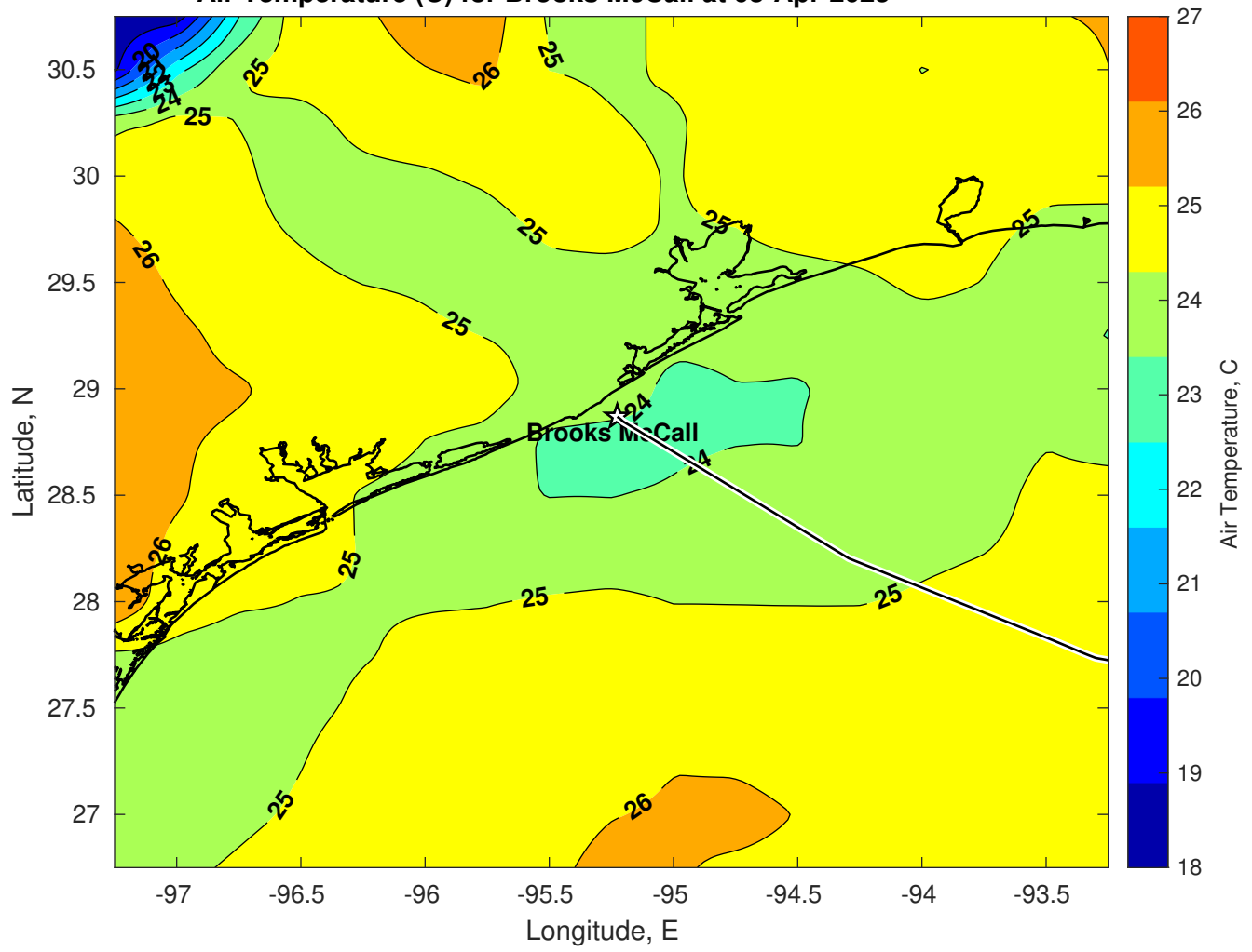
Air Temperature (C) for Brooks McCall at 03-Apr-2025
