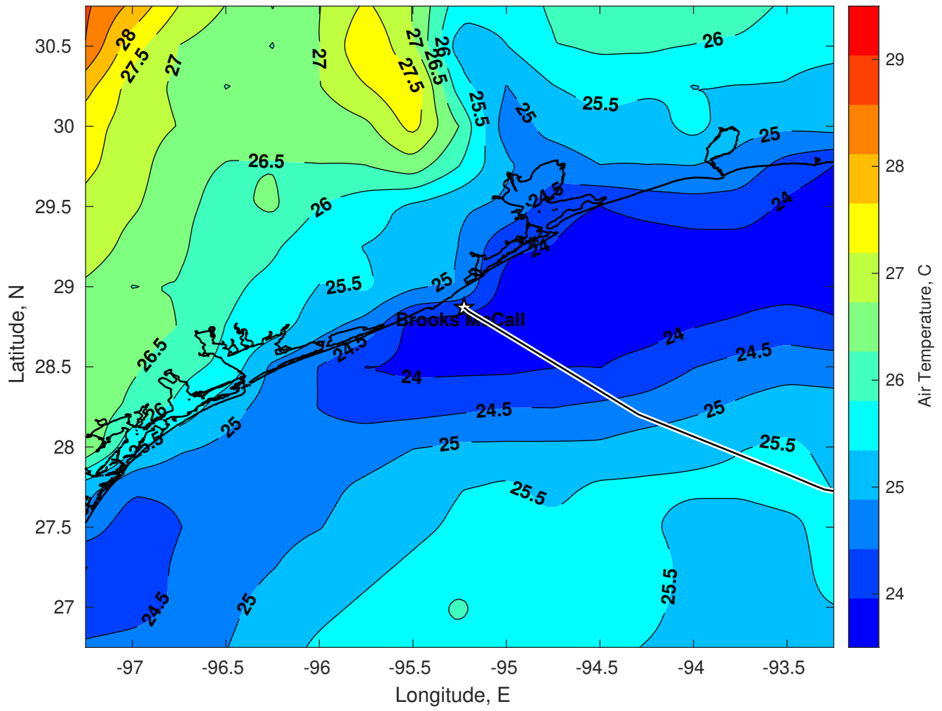
Air Temperature (C) for Brooks McCall at 03-Apr-2025
