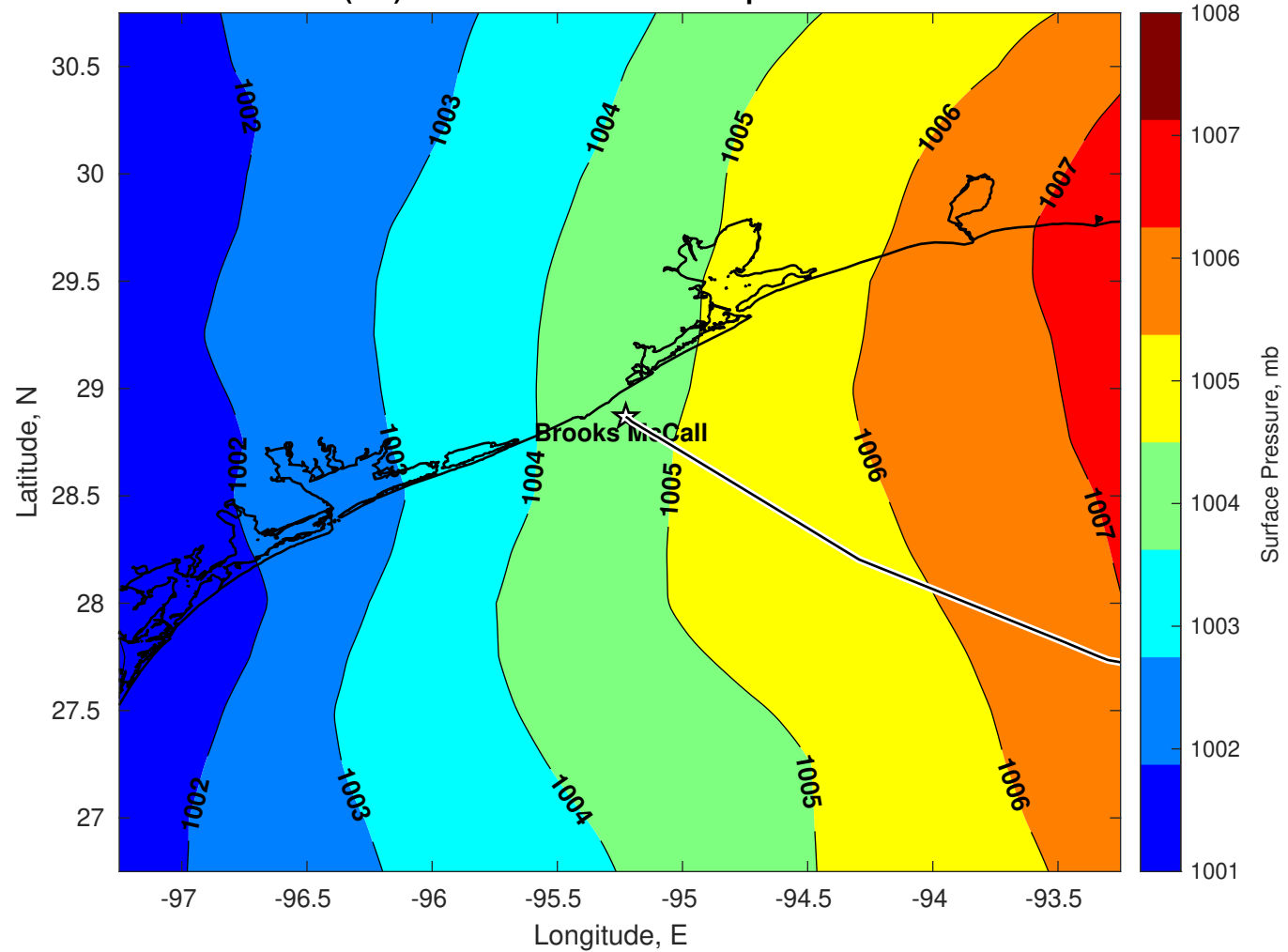
Surface Pressure (mb) for Brooks McCall at 03-Apr-2025 00:00:00
