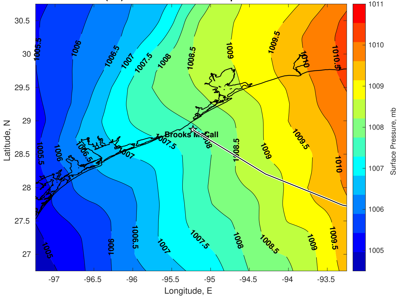
Surface Pressure (mb) for Brooks McCall at 04-Apr-2025 00:00:00
