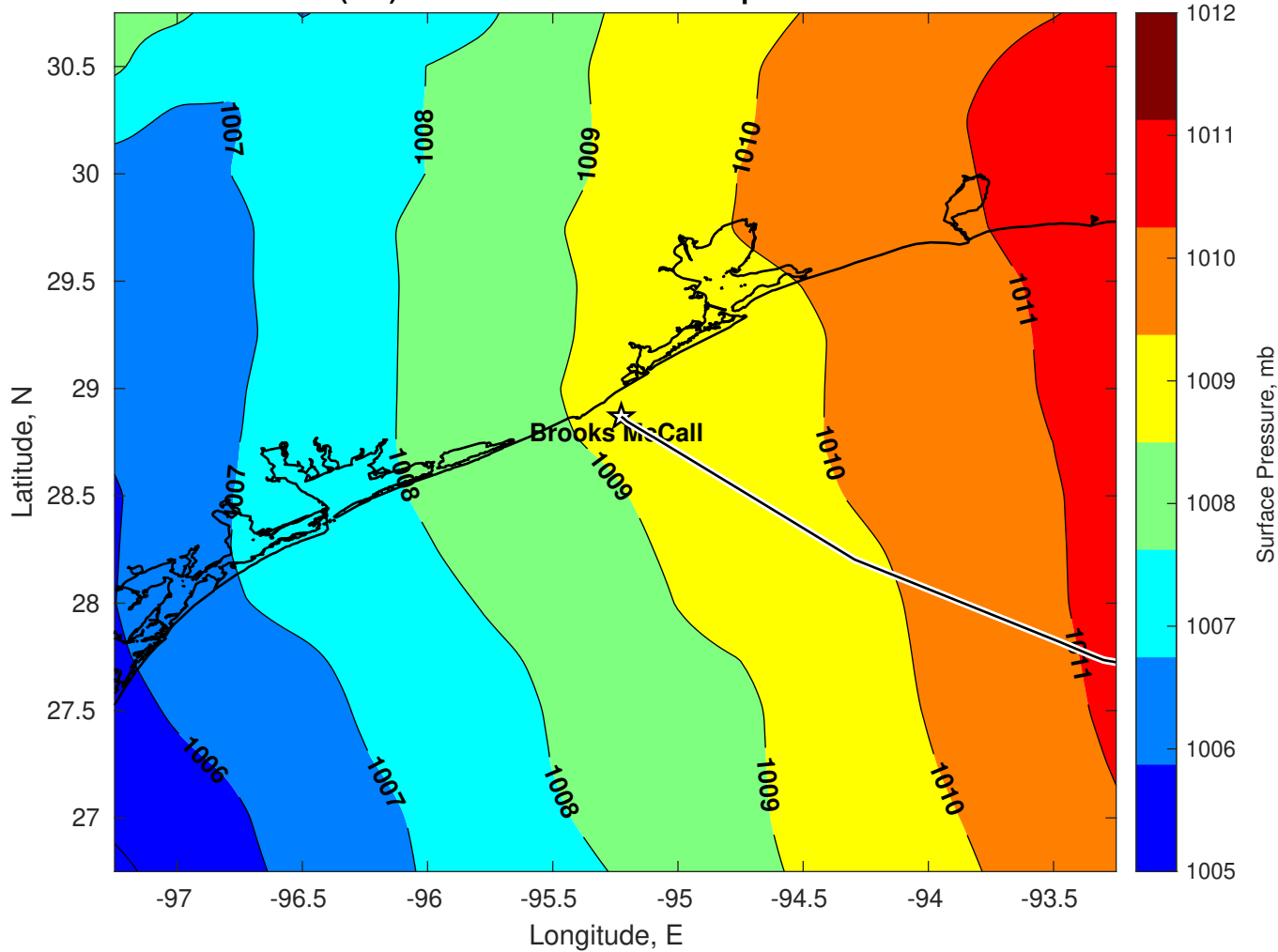
Surface Pressure (mb) for Brooks McCall at 05-Apr-2025 00:00:00
