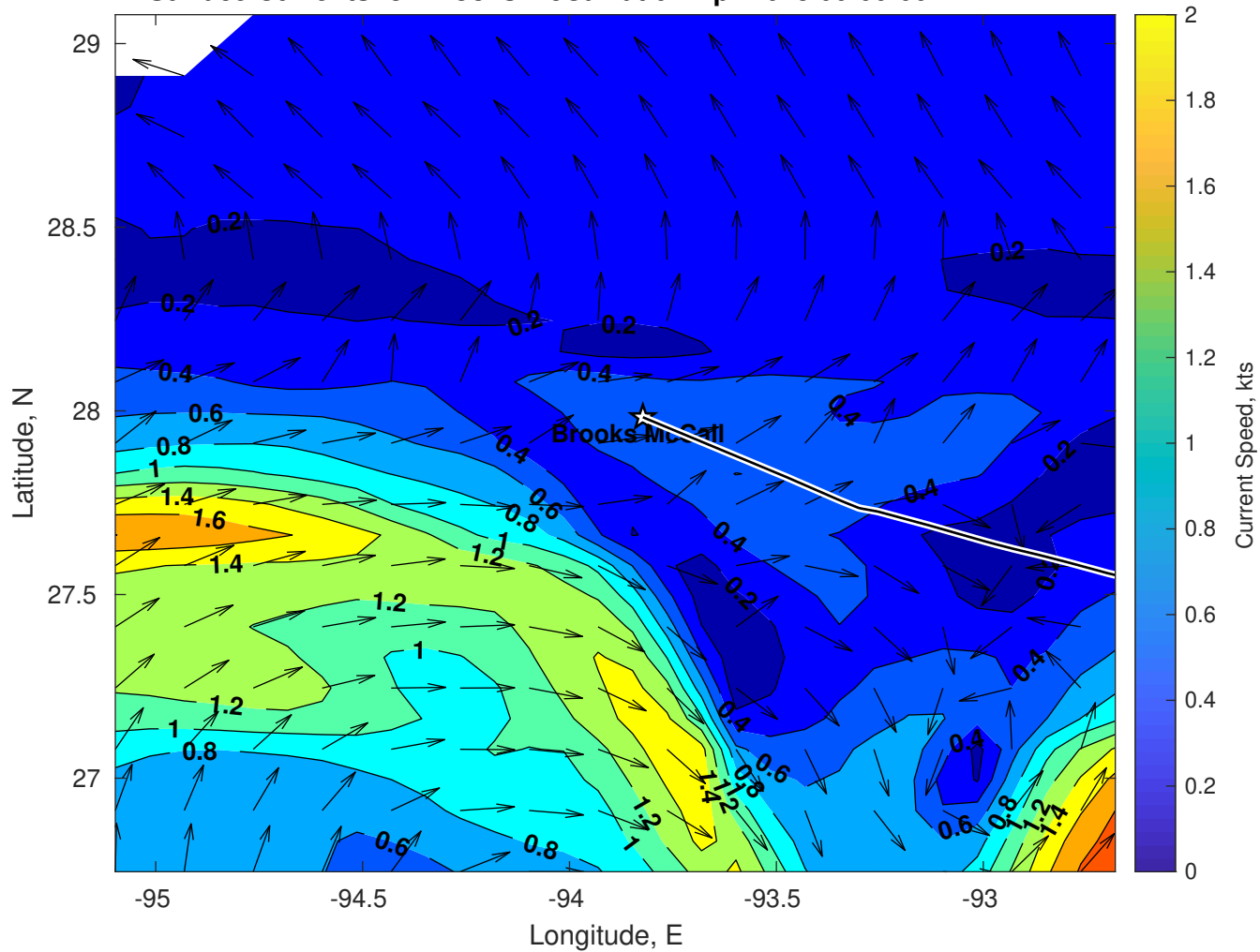
Surface Currents for Brooks McCall at 02-Apr-2025 00:00:00
