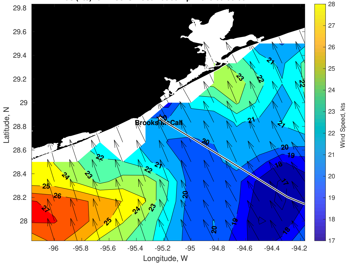
Winds (kts) for Brooks McCall at 03-Apr-2025 09:00:00
