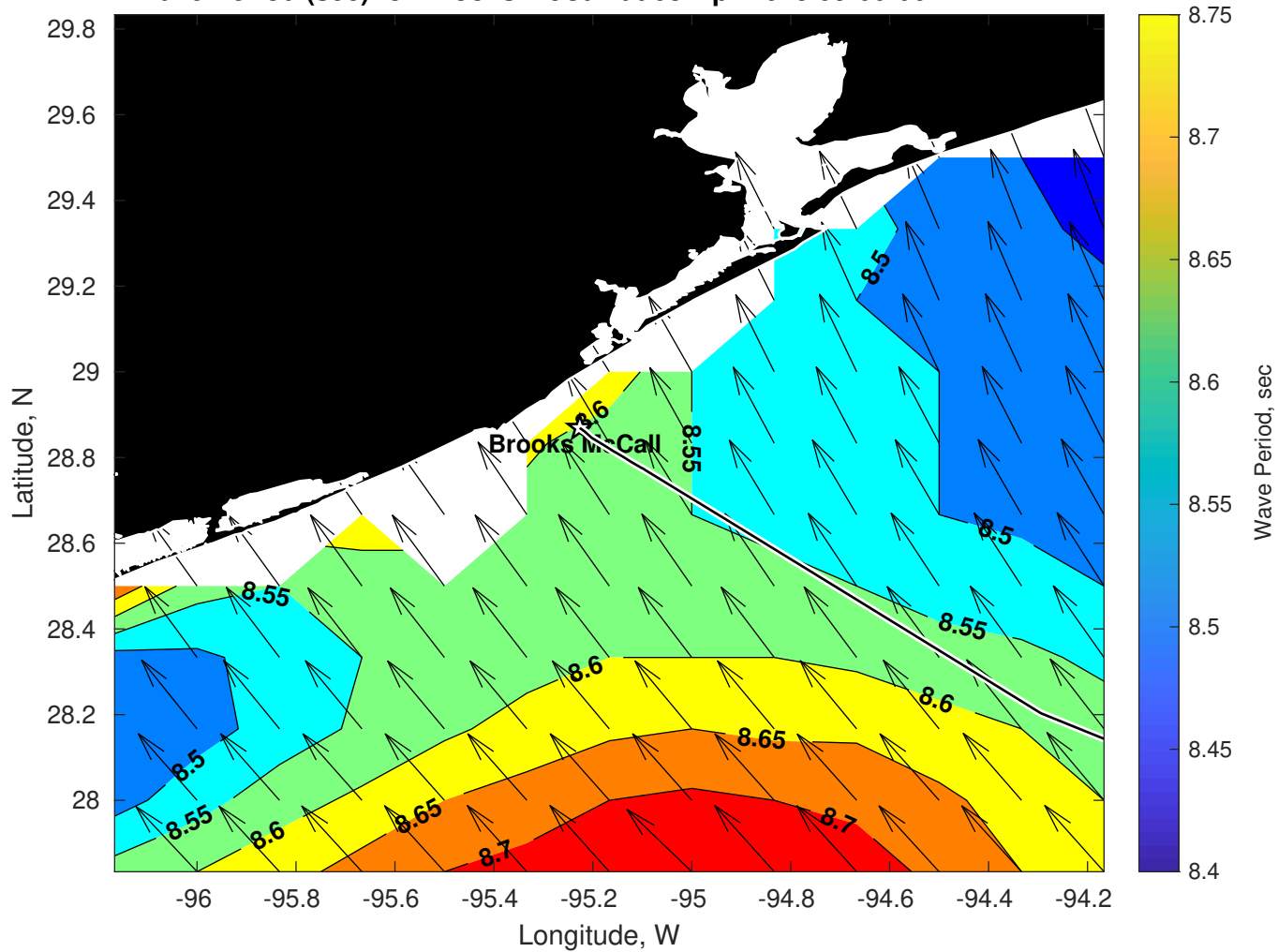
Wave Period (sec) for Brooks McCall at 03-Apr-2025 09:00:00
