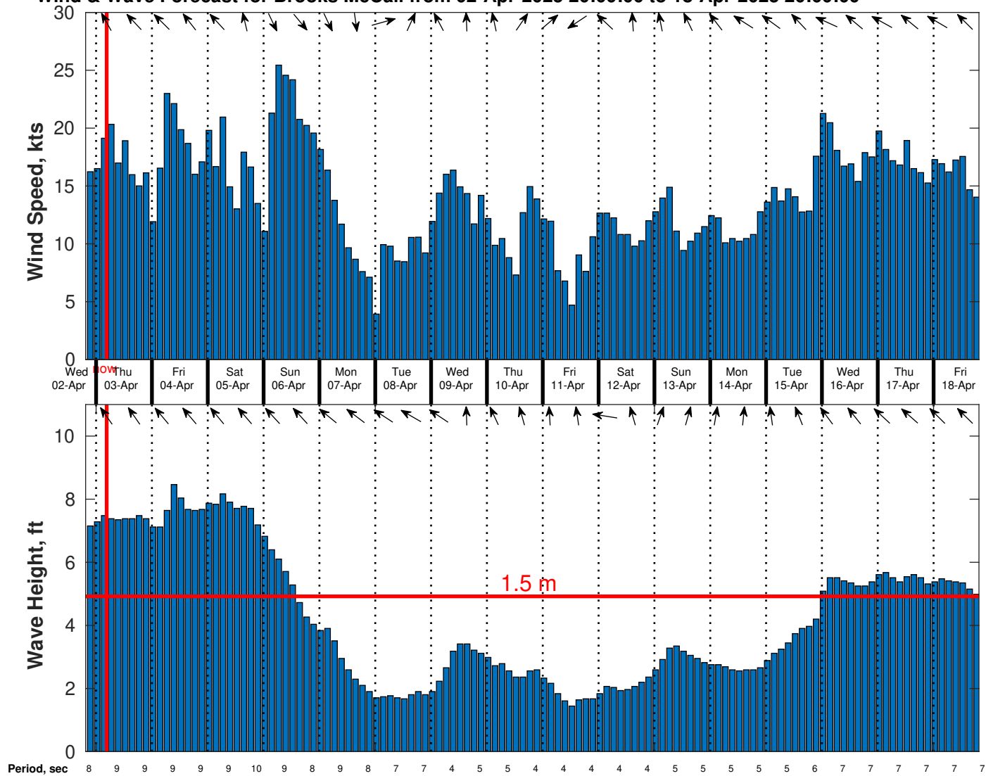
Wind & Wave Forecast for Brooks McCall from 02-Apr-2025 20:00:00 to 18-Apr-2025 20:00:00
