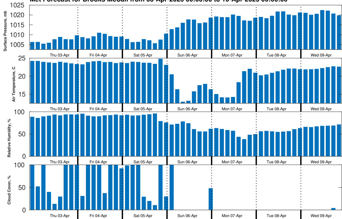
Met Forecast for Brooks McCall from 03-Apr-2025 00:00:00 to 10-Apr-2025 00:00:00
