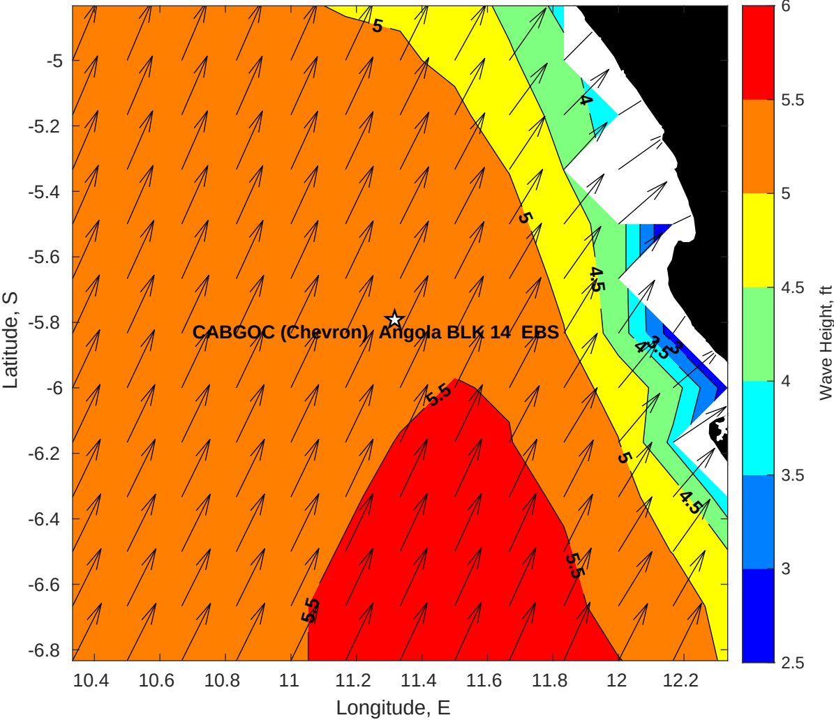
Wave Height (ft) for CABGOC (Chevron) Angola BLK 14 EBS at 03-Apr-2025 09:00:00
