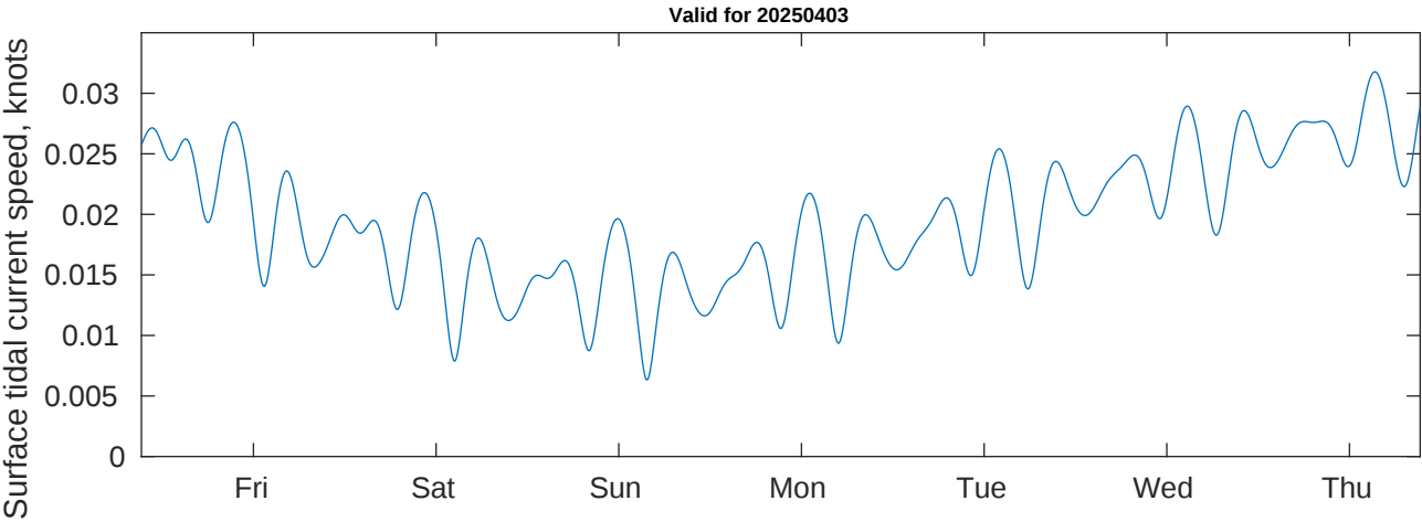
Tidal Currents and Heights for CABGOC (Chevron) Angola BLK 14 EBS at 20250403
