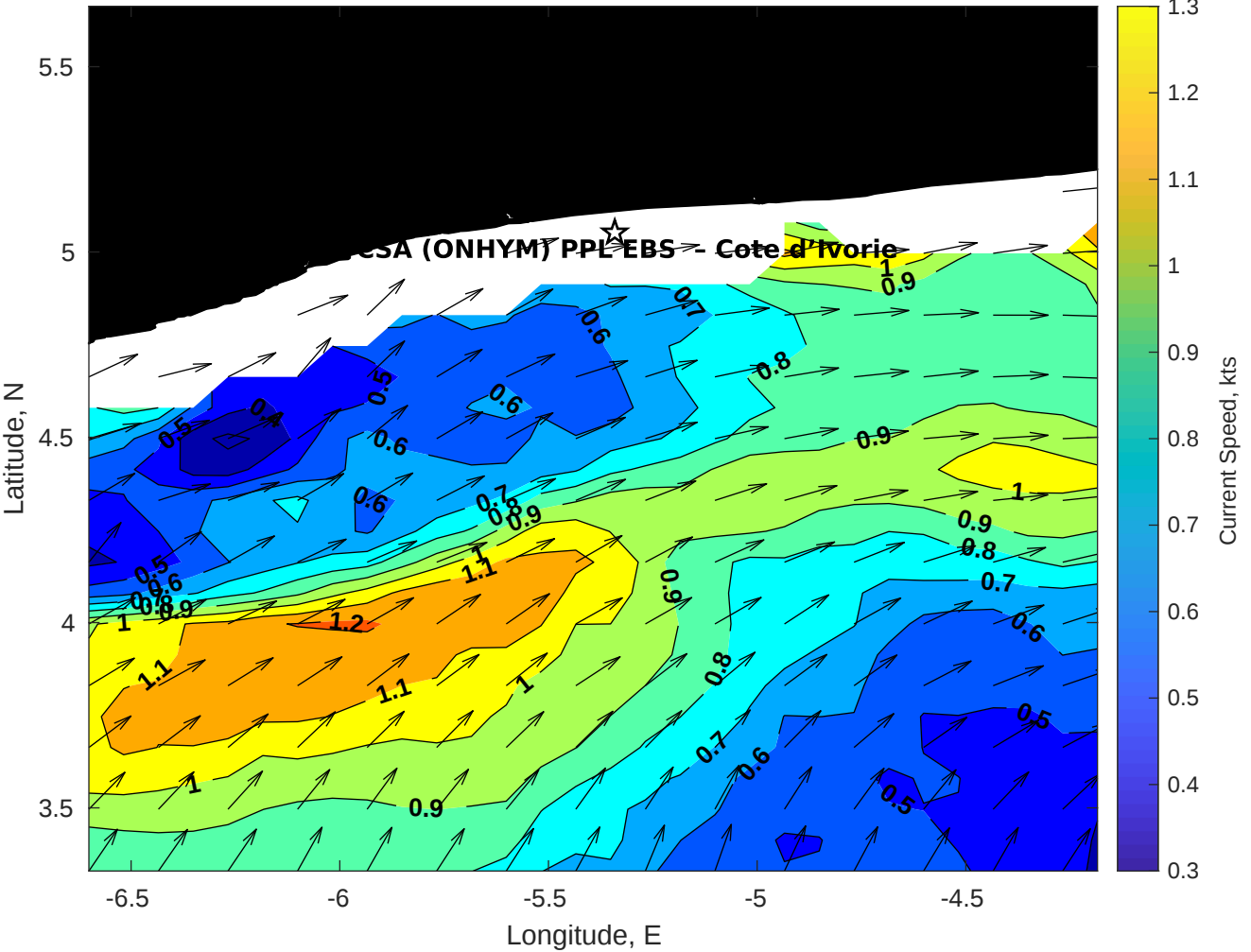
Surface Currents for CSA (ONHYM) PPL EBS - Cote d'Ivoire at 02-Apr-2025 00:00:00
