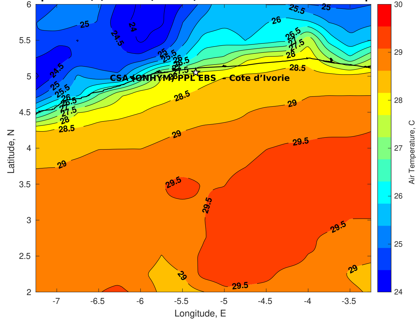
Air Temperature (C) for CSA (ONHYM) PPL EBS - Cote d'Ivoire at 03-Apr-2025
