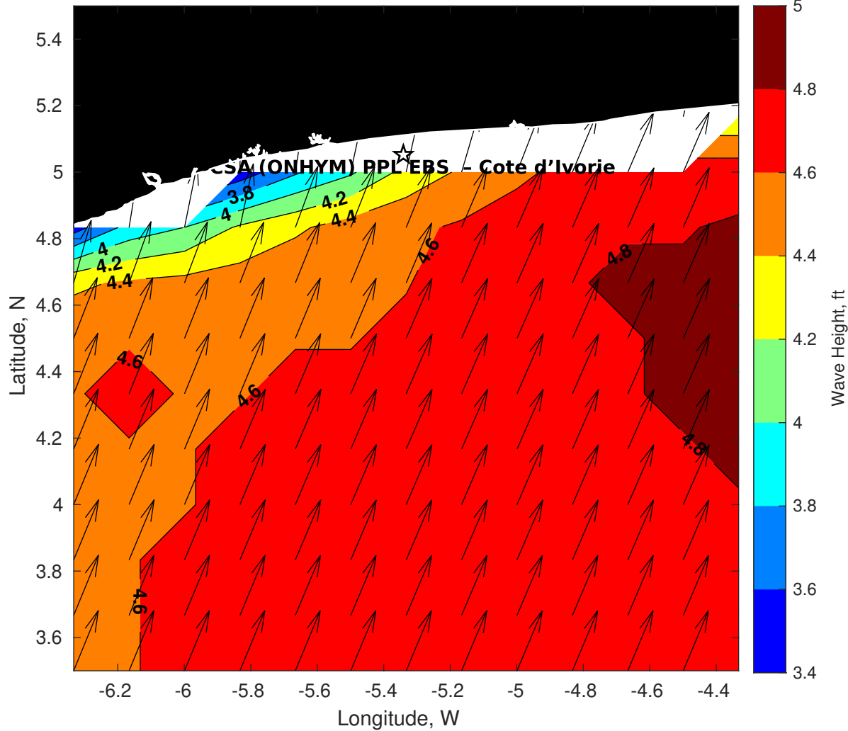
Wave Height (ft) for CSA (ONHYM) PPL EBS - Cote d'Ivoire at 03-Apr-2025 09:00:00
