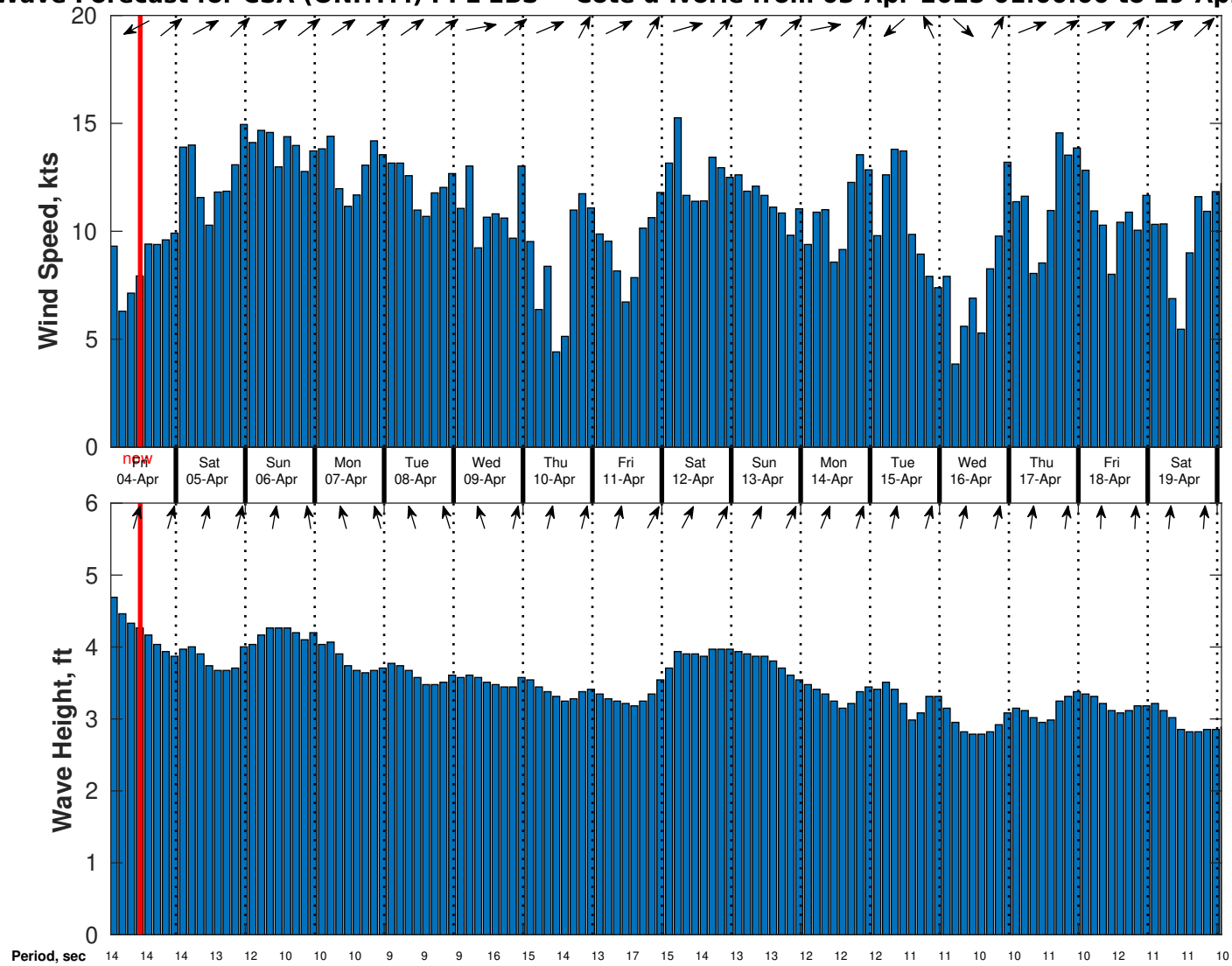
Wind & Wave Forecast for CSA (ONHYM) PPL EBS - Cote d'Ivoire from 03-Apr-2025 01:00:00 to 19-Apr-2025 01:00:00
