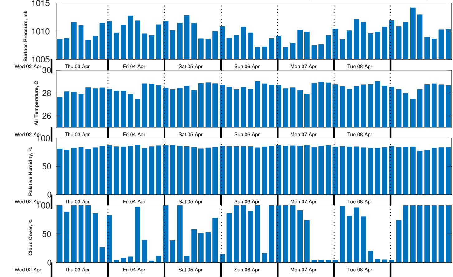
Met Forecast for CSA (ONHYM) PPL EBS - Cote d'Ivoire from 03-Apr-2025 00:00:00 to 10-Apr-2025 00:00:00
