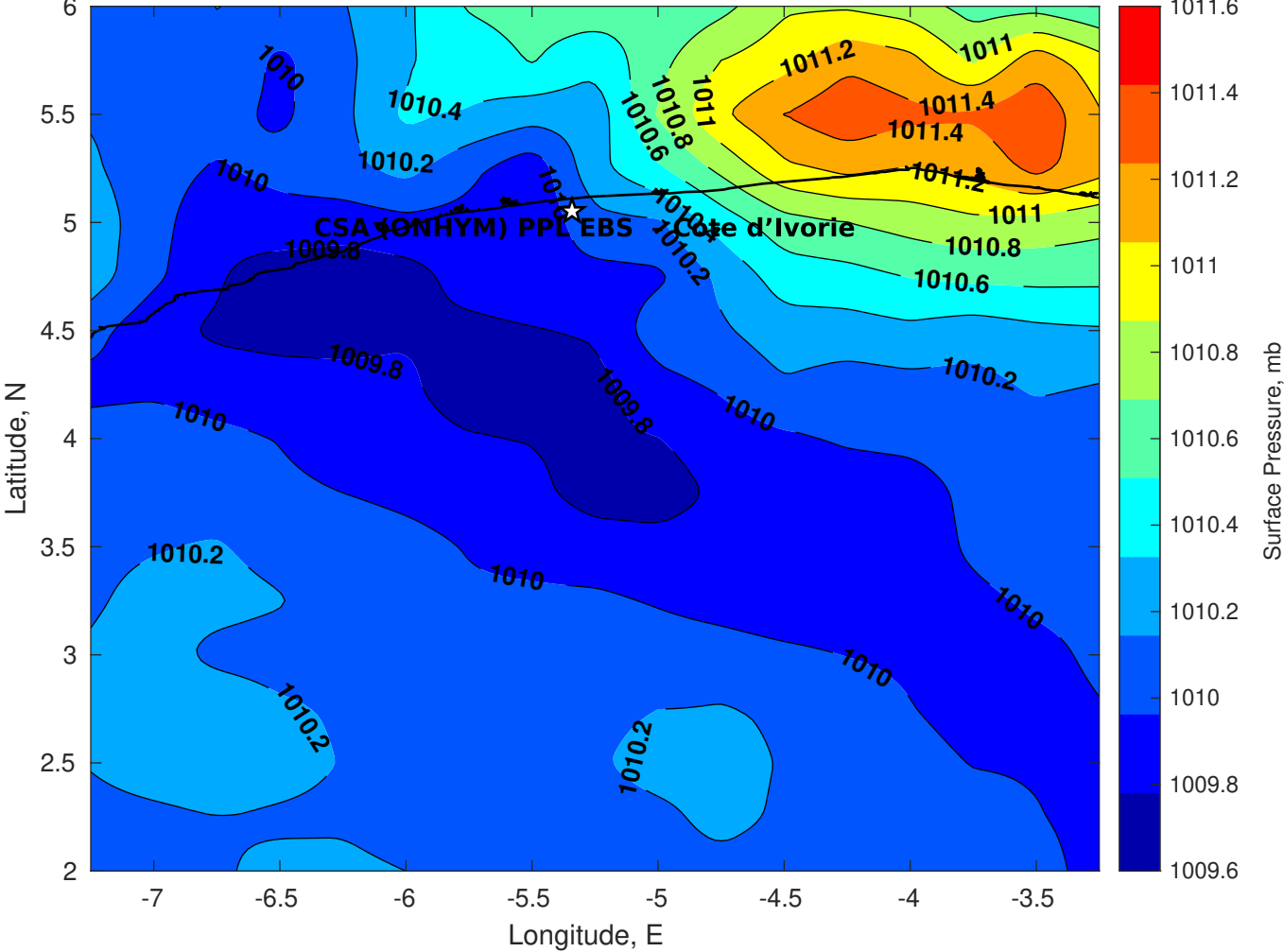
Surface Pressure (mb) for CSA (ONHYM) PPL EBS - Cote d'Ivoire at 03-Apr-2025 00:00:00
