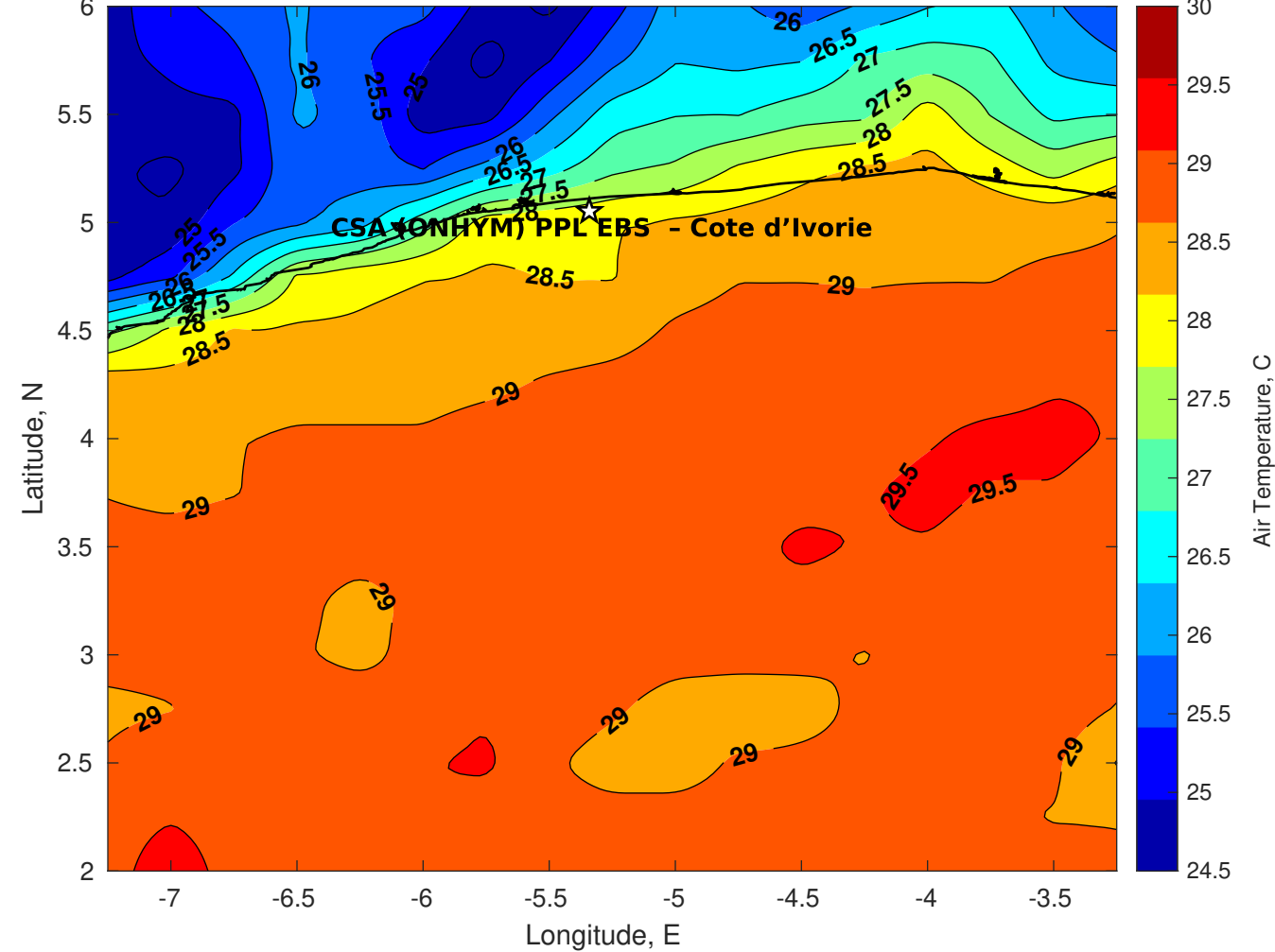
Air Temperature (C) for CSA (ONHYM) PPL EBS - Cote d'Ivoire at 03-Apr-2025
