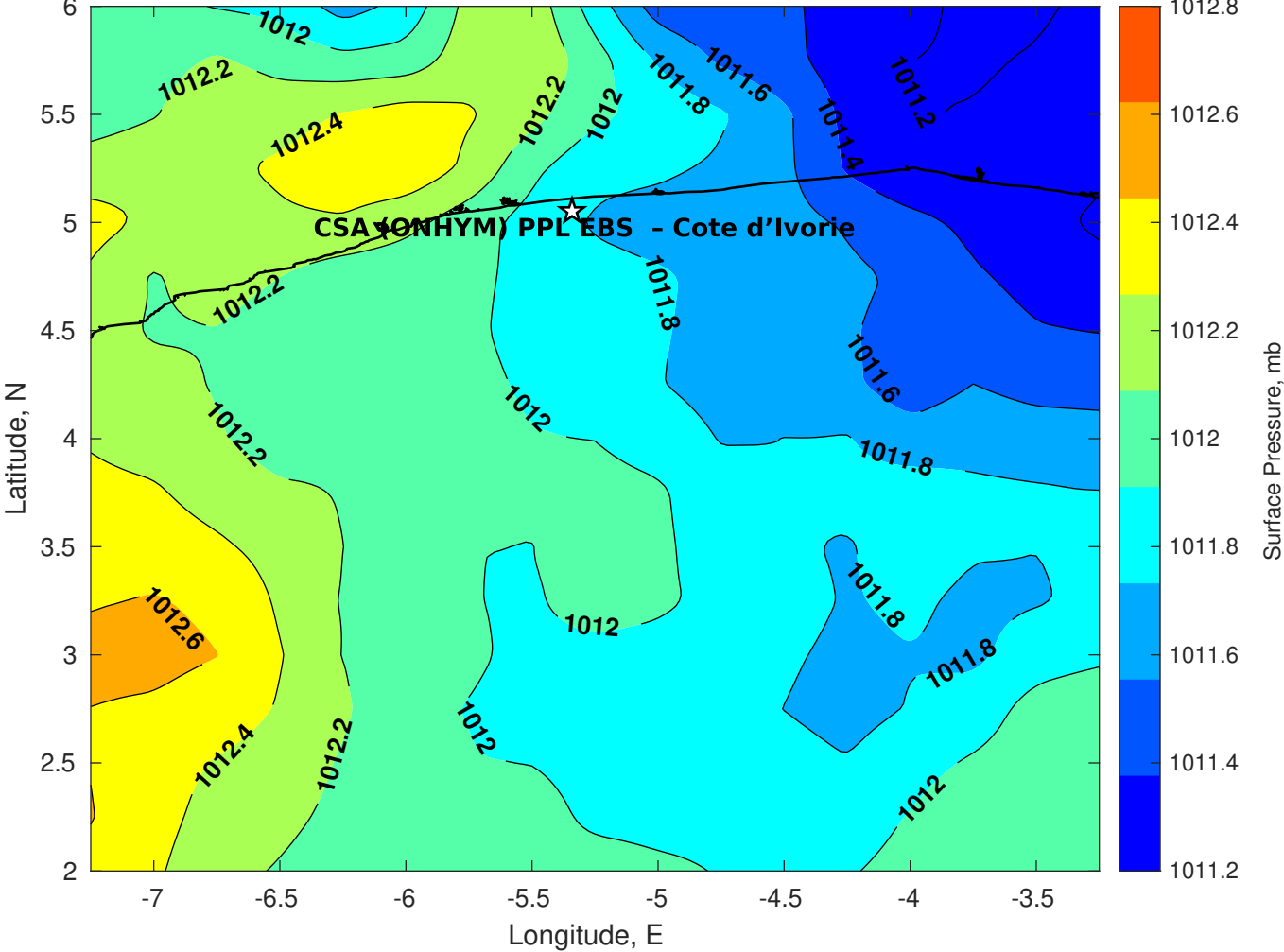
Surface Pressure (mb) for CSA (ONHYM) PPL EBS - Cote d'Ivoire at 04-Apr-2025 00:00:00
