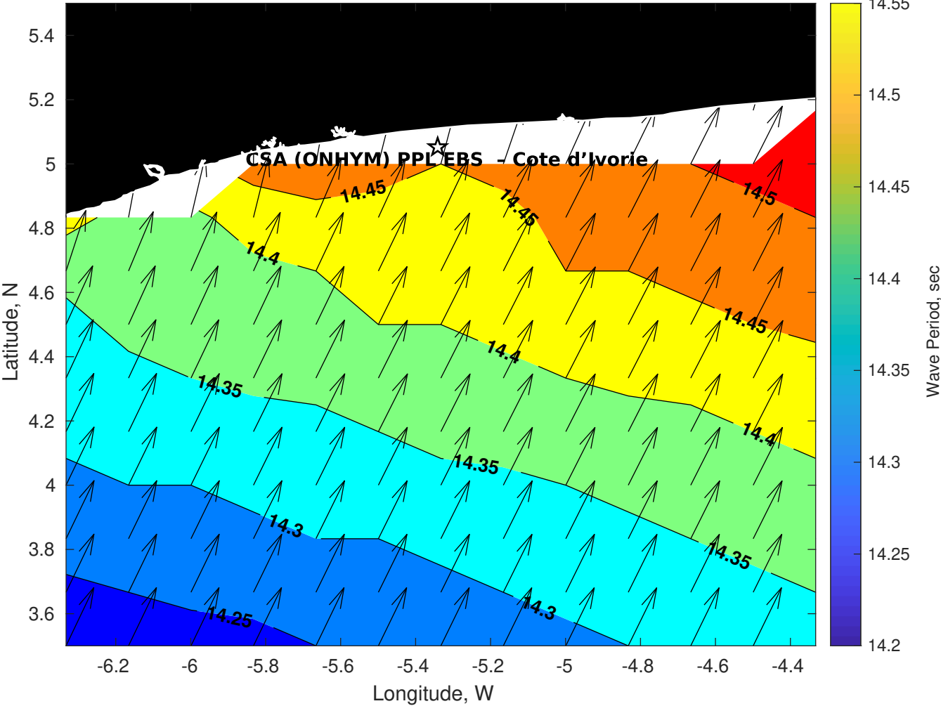
Wave Period (sec) for CSA (ONHYM) PPL EBS - Cote d'Ivoire at 03-Apr-2025 09:00:00
