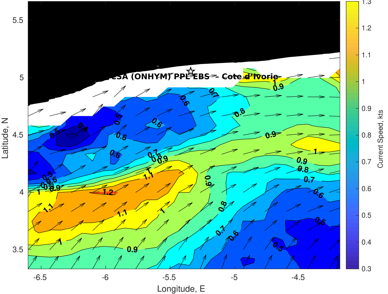
Surface Currents for CSA (ONHYM) PPL EBS - Cote d'Ivoire at 02-Apr-2025 00:00:00
