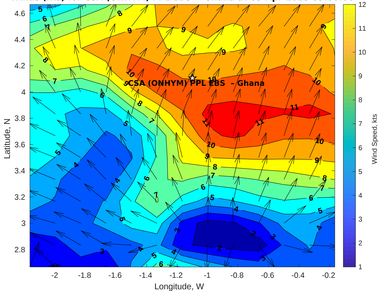
Winds (kts) for CSA (ONHYM) PPL EBS - Ghana at 03-Apr-2025 09:00:00
