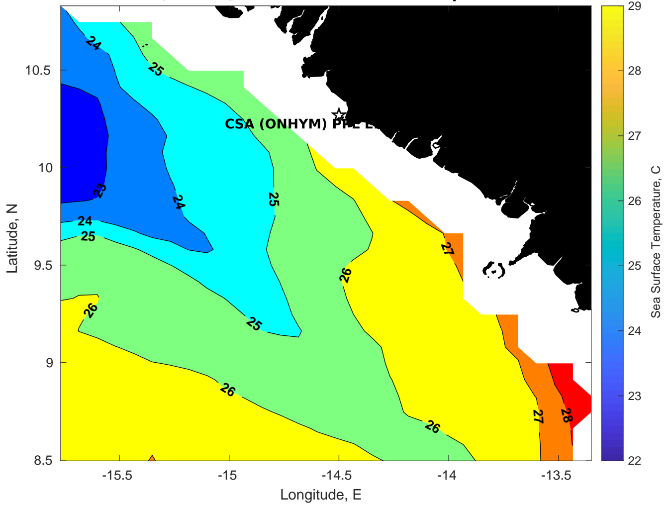
SST for CSA (ONHYM) PPL EBS - Guinea at 02-Apr-2025 00:00:00
