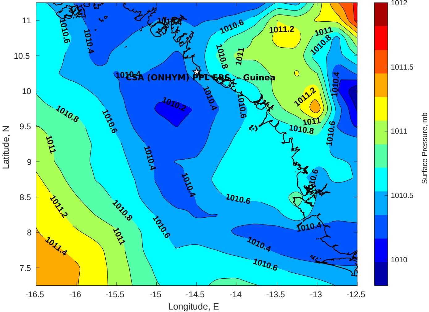
Surface Pressure (mb) for CSA (ONHYM) PPL EBS - Guinea at 03-Apr-2025 00:00:00
