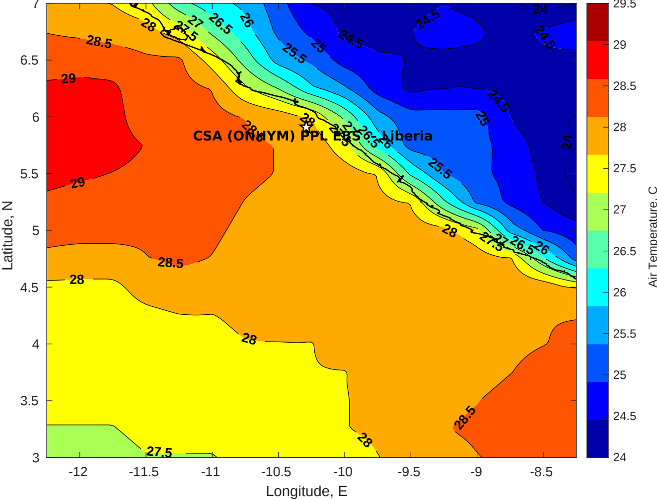
Air Temperature (C) for CSA (ONHYM) PPL EBS - Liberia at 03-Apr-2025
