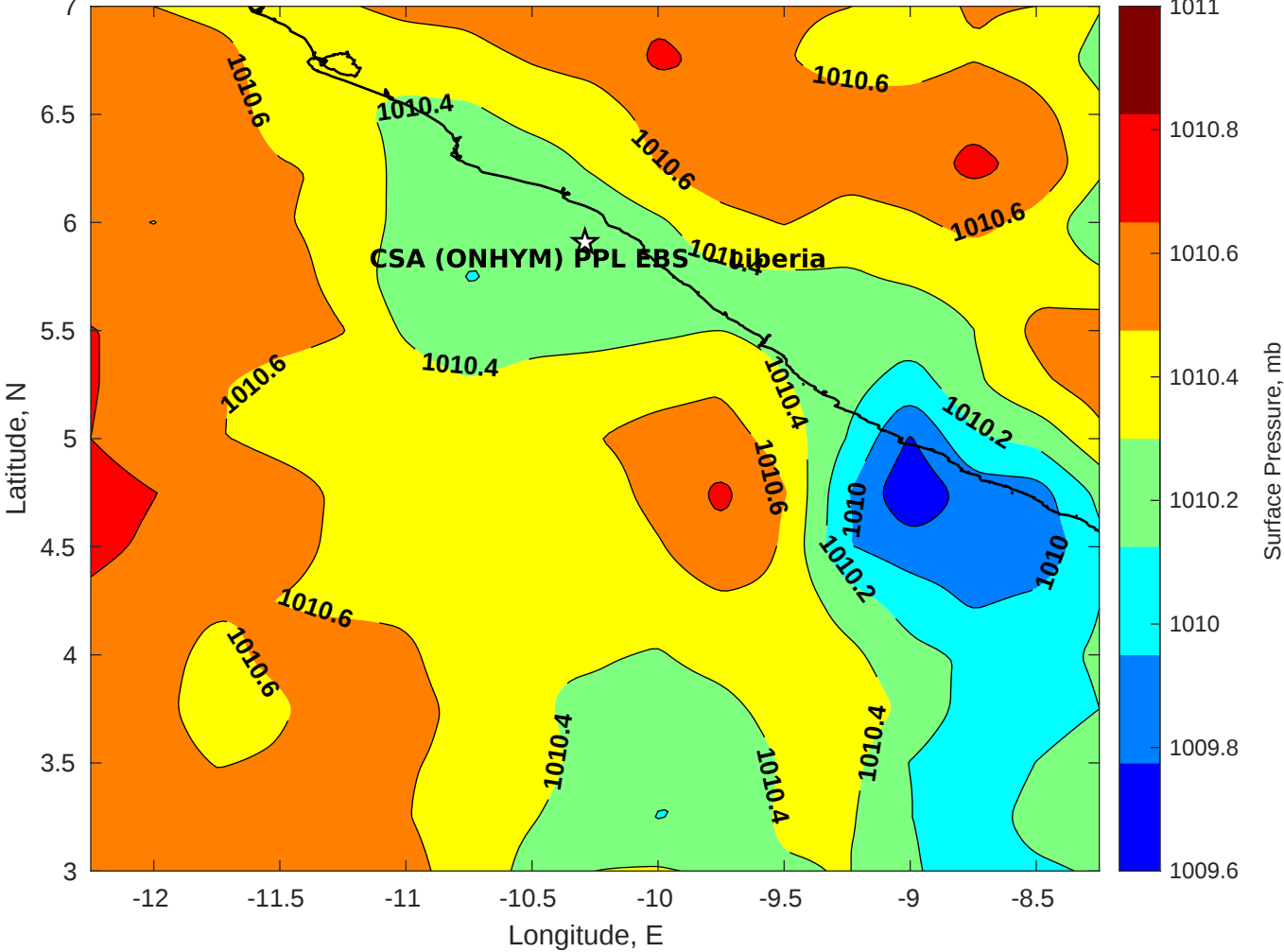
Surface Pressure (mb) for CSA (ONHYM) PPL EBS - Liberia at 03-Apr-2025 00:00:00
