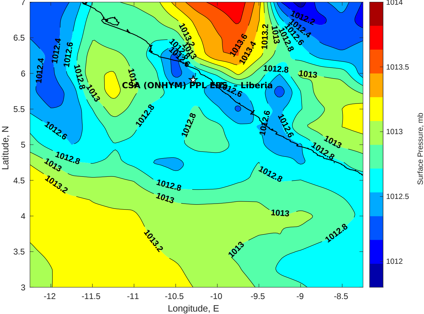
Surface Pressure (mb) for CSA (ONHYM) PPL EBS - Liberia at 04-Apr-2025 00:00:00
