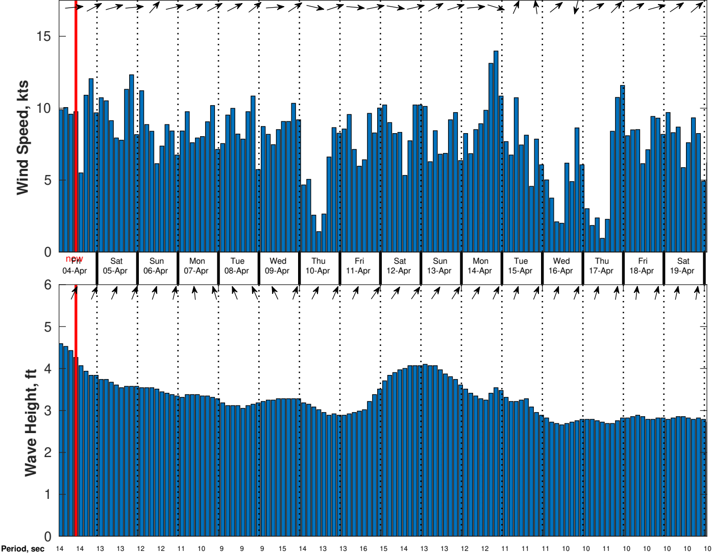
Wind & Wave Forecast for CSA (ONHYM) PPL EBS - Liberia from 03-Apr-2025 01:00:00 to 19-Apr-2025 01:00:00
