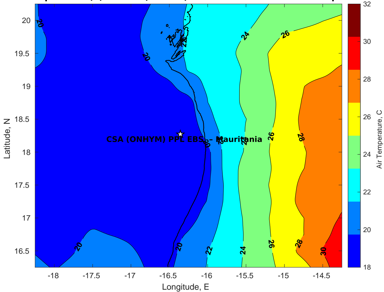
Air Temperature (C) for CSA (ONHYM) PPL EBS - Mauritania at 03-Apr-2025
