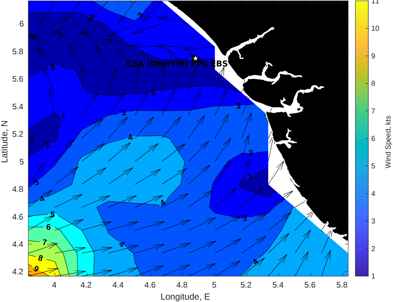
Winds (kts) for CSA (ONHYM) PPL EBS - Nigeria at 03-Apr-2025 09:00:00
