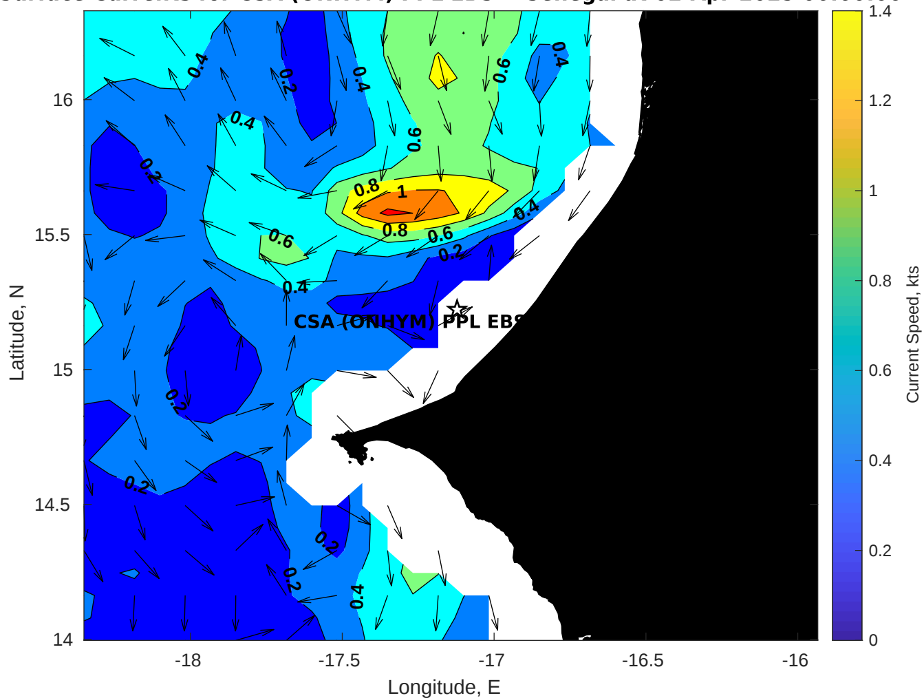
Surface Currents for CSA (ONHYM) PPL EBS - Senegal at 02-Apr-2025 00:00:00
