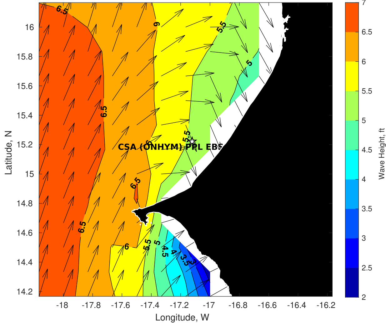
Wave Height (ft) for CSA (ONHYM) PPL EBS - Senegal at 03-Apr-2025 09:00:00
