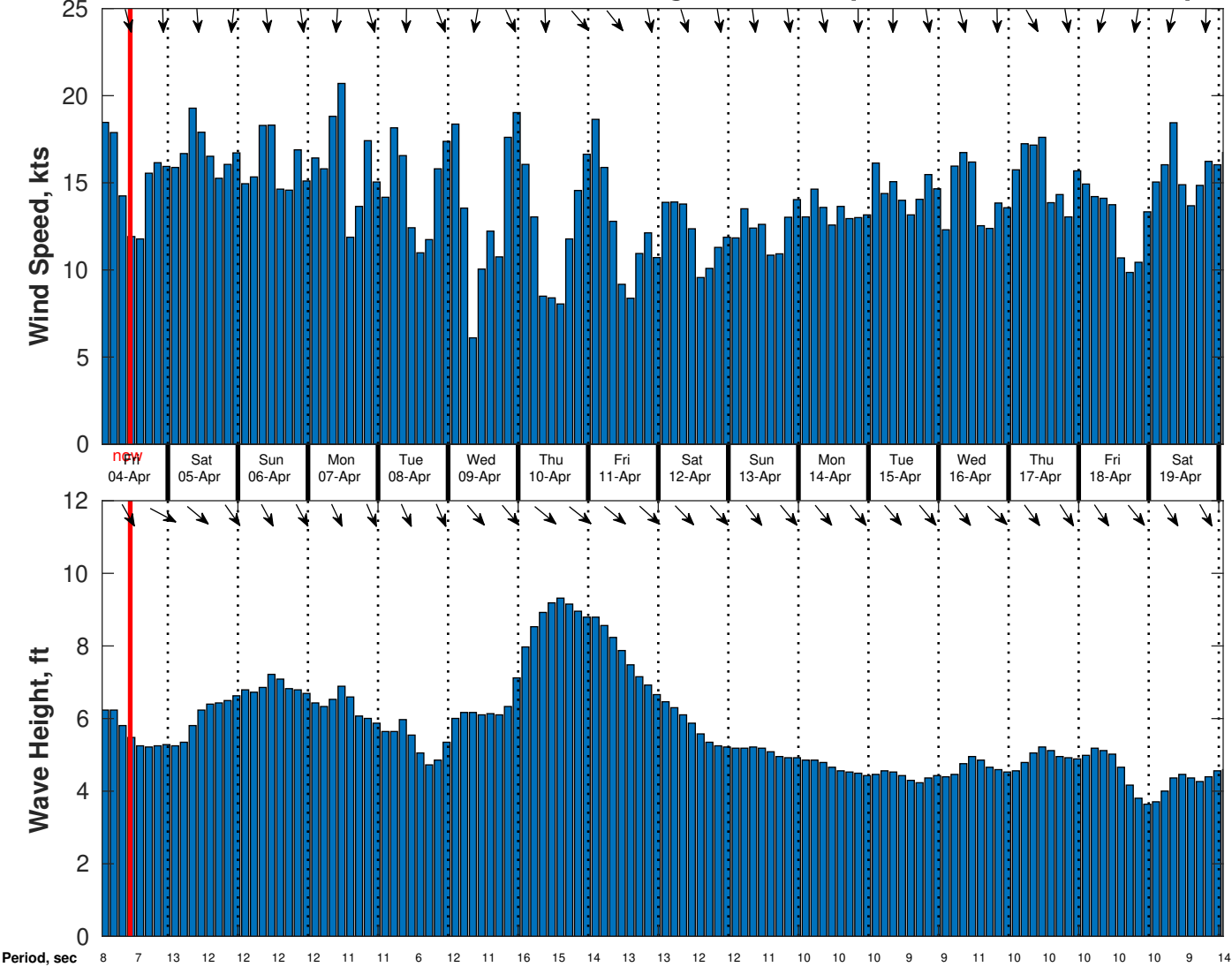
Wind & Wave Forecast for CSA (ONHYM) PPL EBS - Senegal from 03-Apr-2025 01:00:00 to 19-Apr-2025 01:00:00
