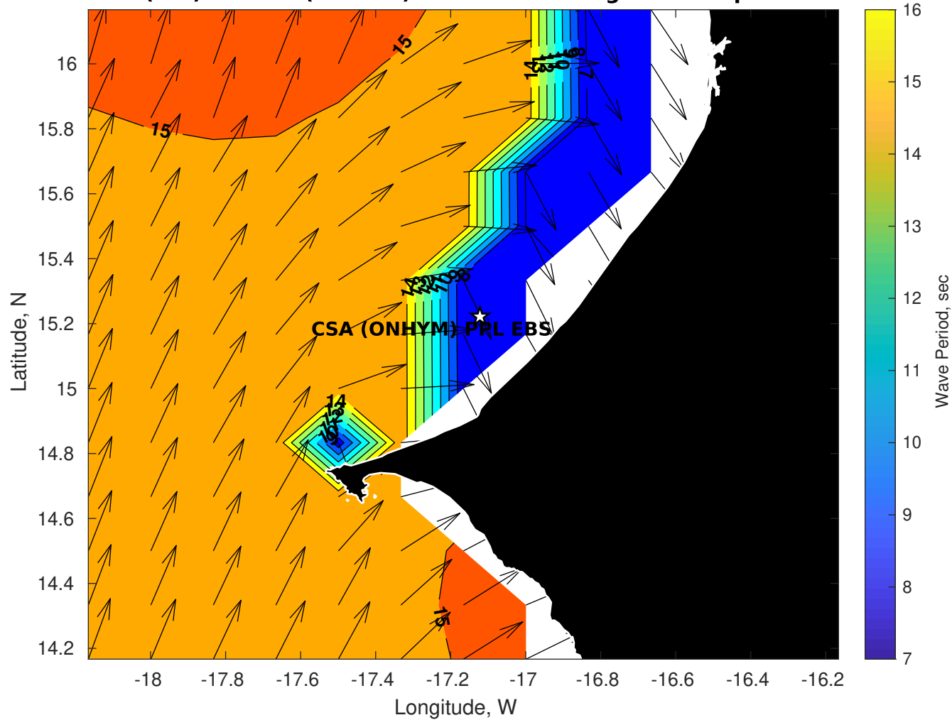
Wave Period (sec) for CSA (ONHYM) PPL EBS - Senegal at 03-Apr-2025 09:00:00
