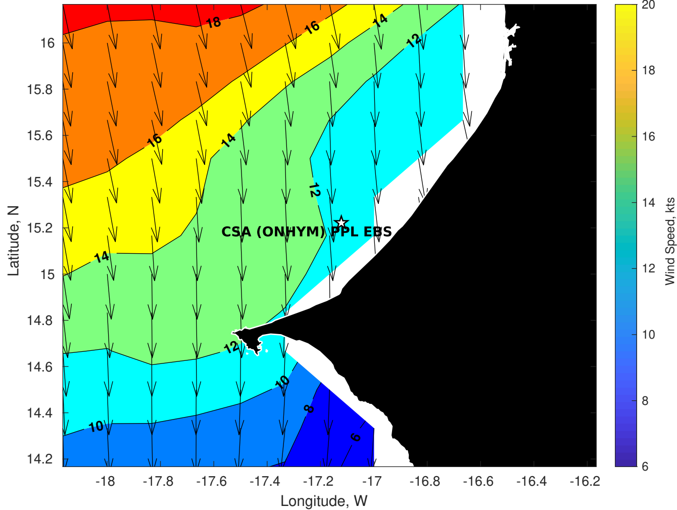
Winds (kts) for CSA (ONHYM) PPL EBS - Senegal at 03-Apr-2025 09:00:00
