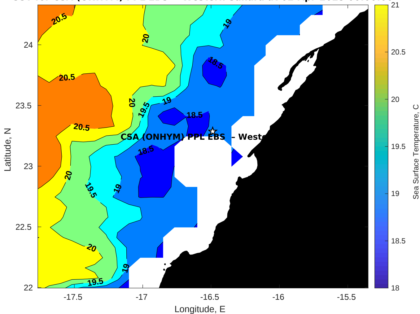
SST for CSA (ONHYM) PPL EBS - Western Sahara at 02-Apr-2025 00:00:00
