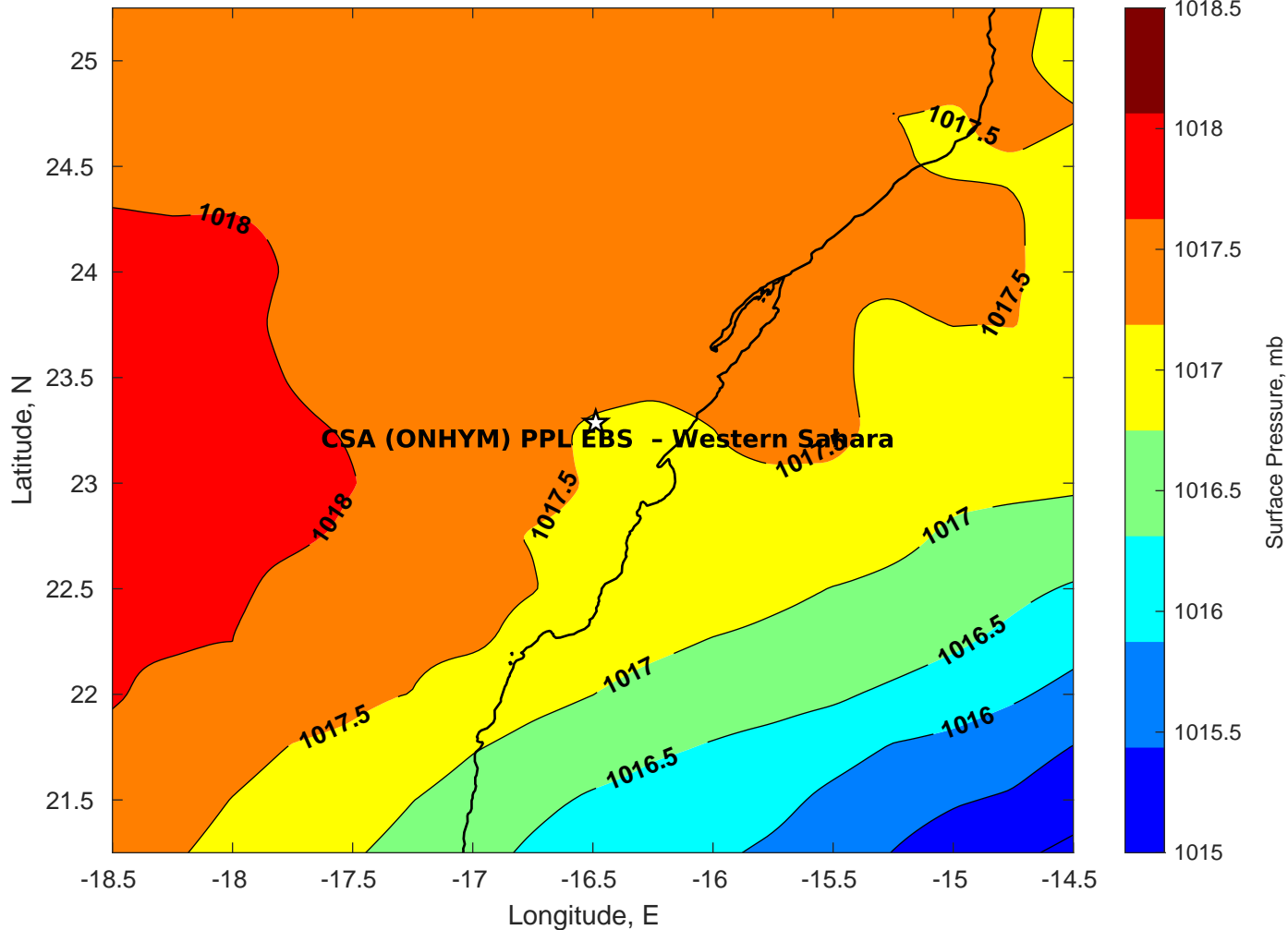
Surface Pressure (mb) for CSA (ONHYM) PPL EBS - Western Sahara at 05-Apr-2025 00:00:00
