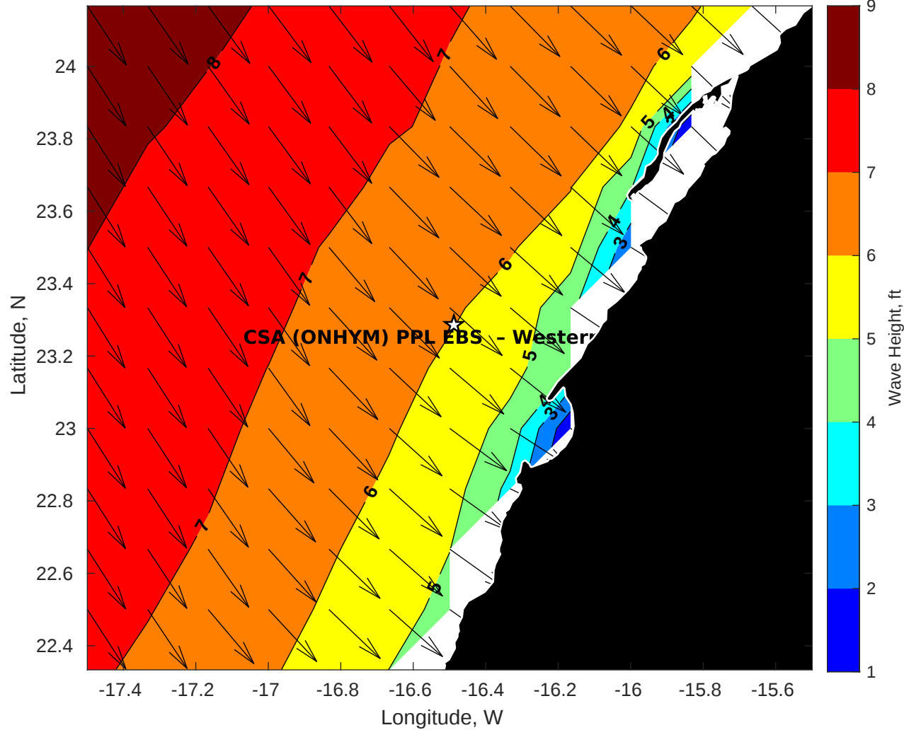
Wave Height (ft) for CSA (ONHYM) PPL EBS - Western Sahara at 03-Apr-2025 09:00:00
