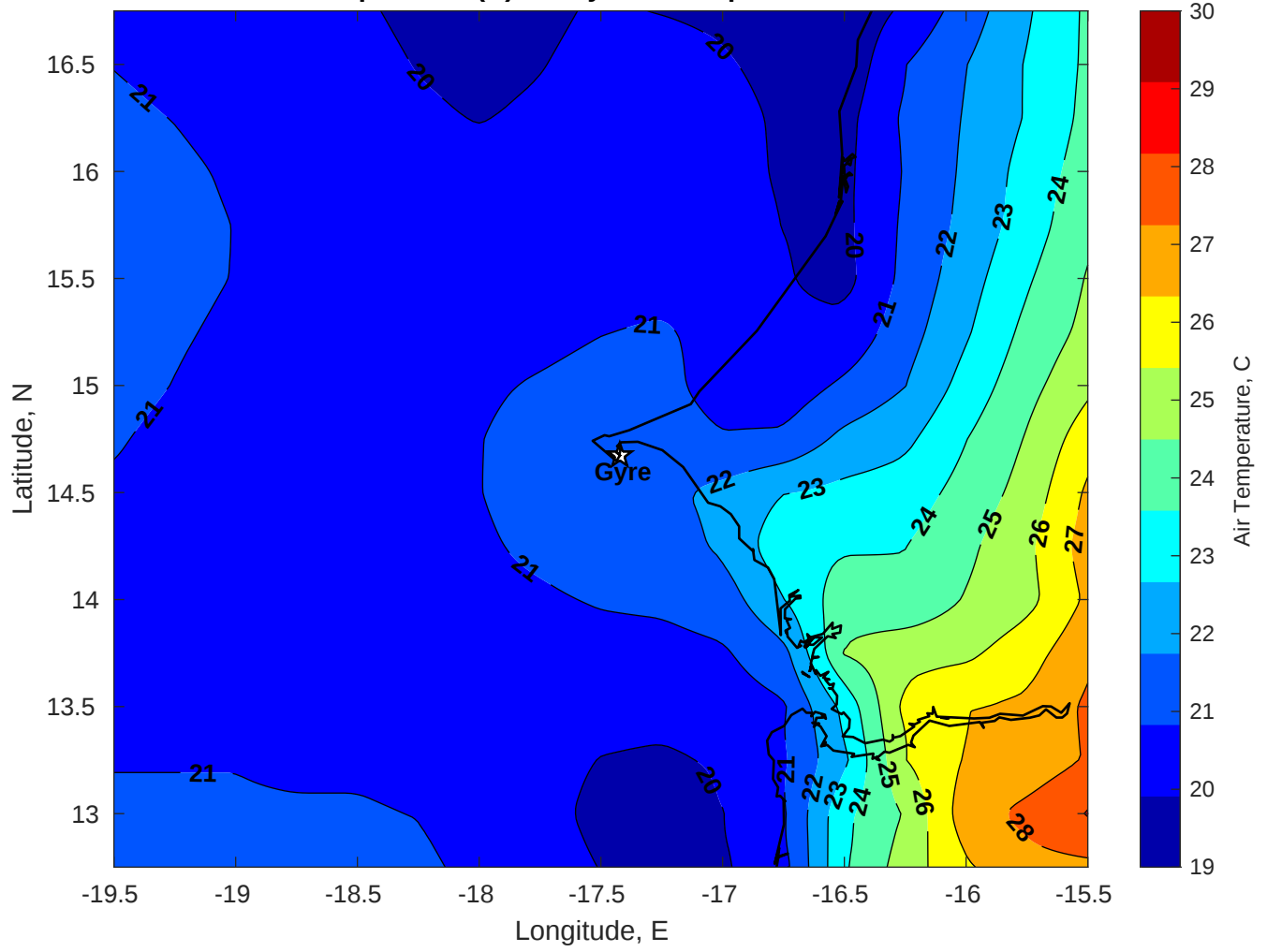
Air Temperature (C) for Gyre at 03-Apr-2025
