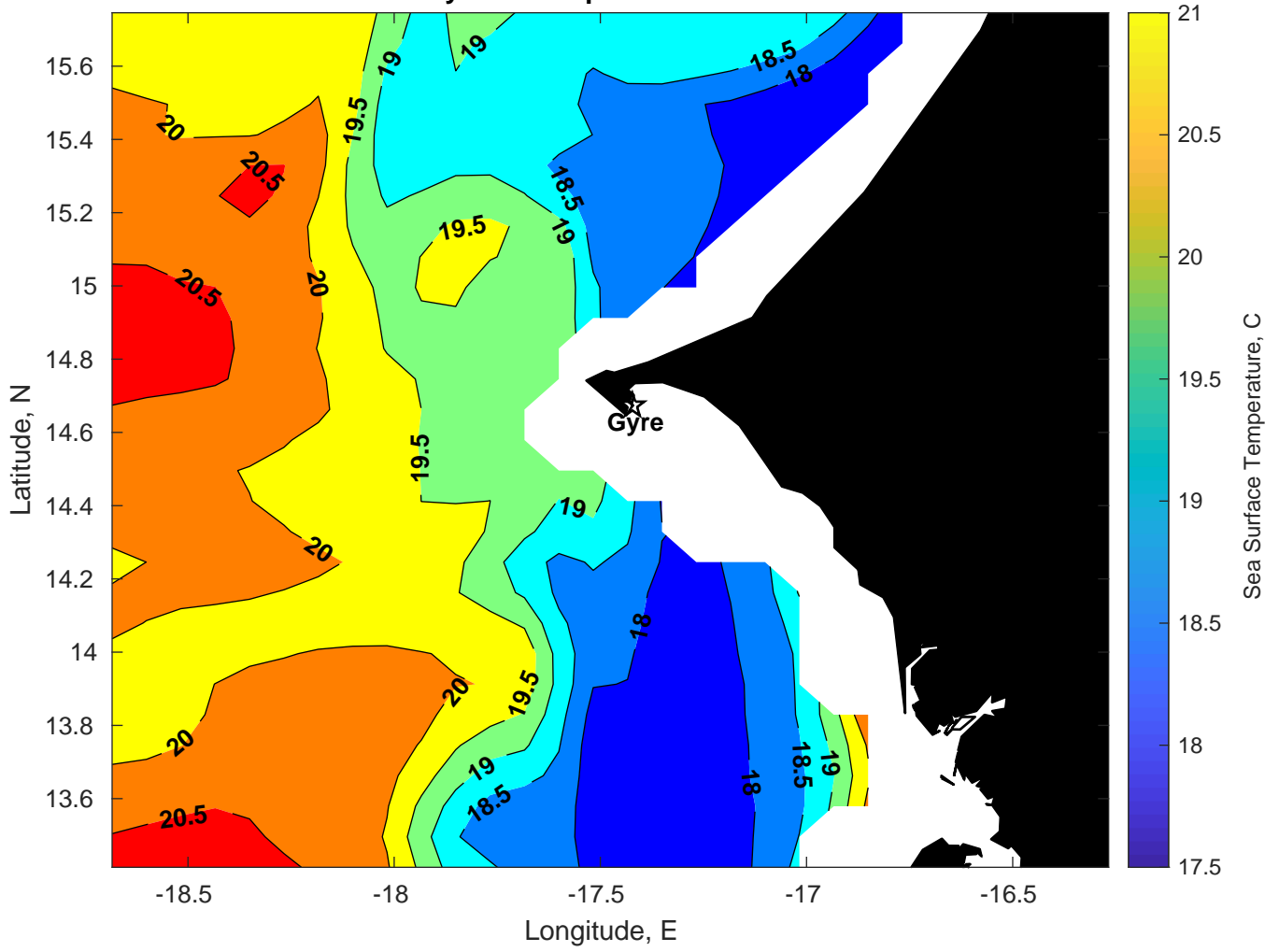
SST for Gyre at 02-Apr-2025 00:00:00
