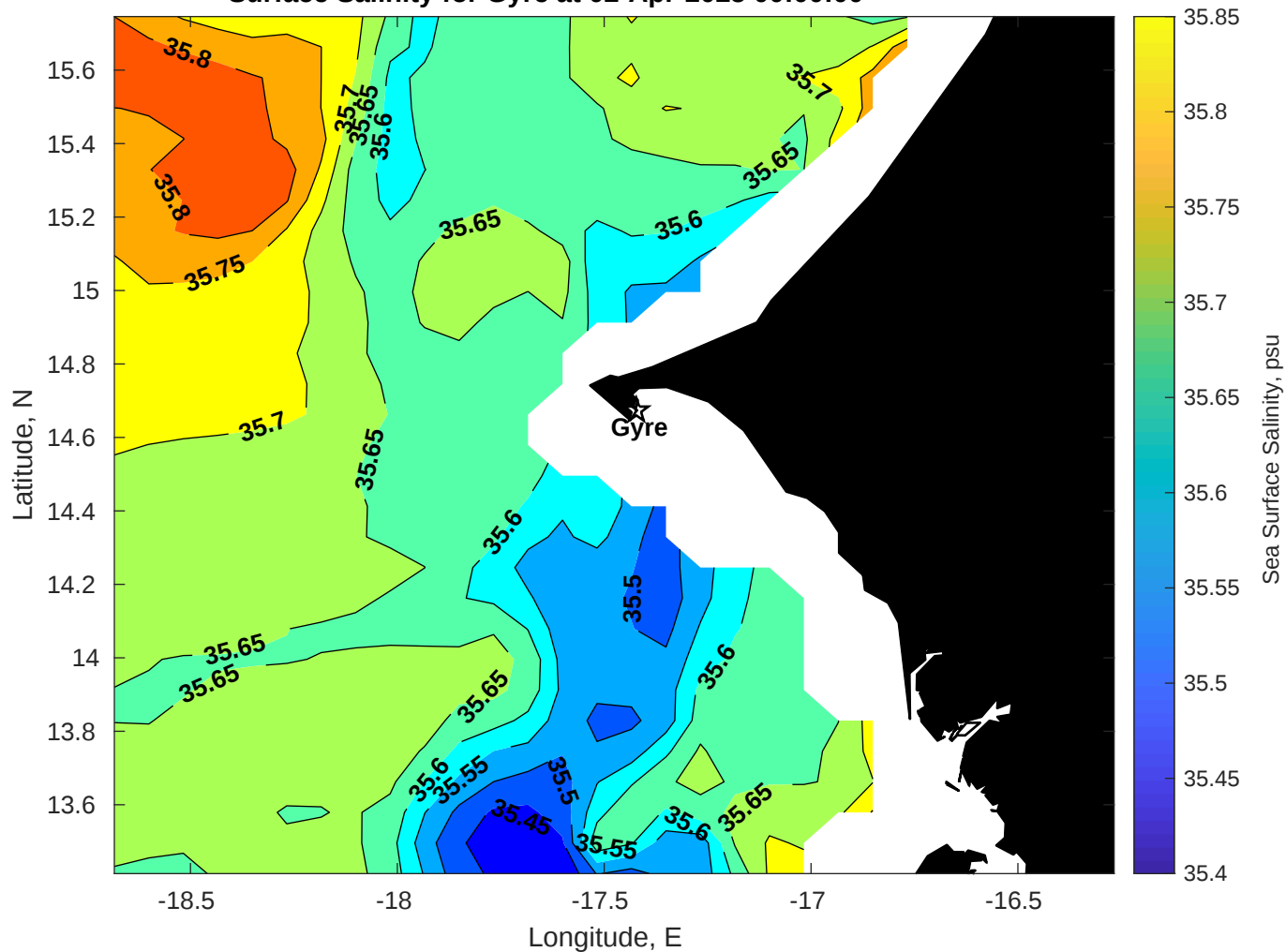
Surface Salinity for Gyre at 02-Apr-2025 00:00:00
