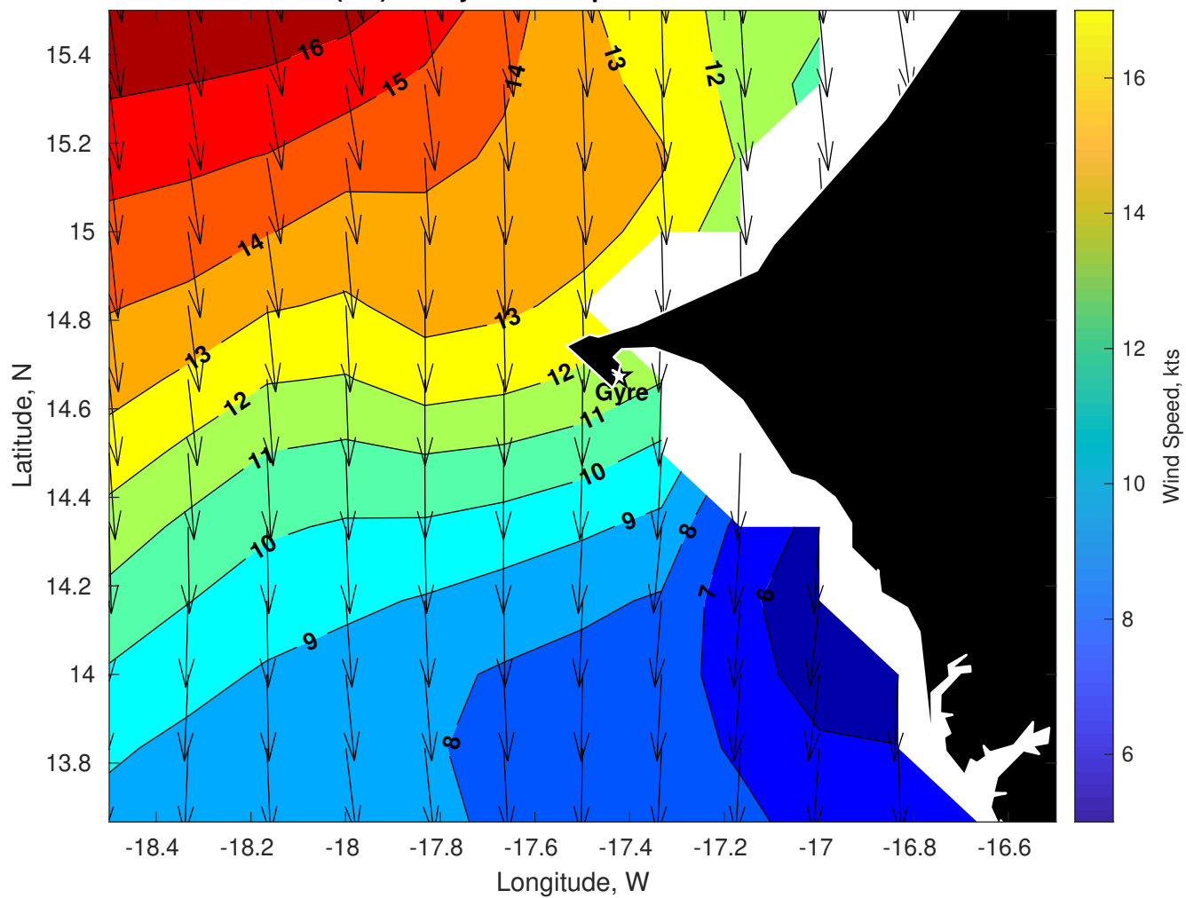
Winds (kts) for Gyre at 03-Apr-2025 09:00:00
