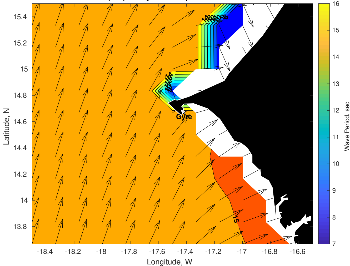
Wave Period (sec) for Gyre at 03-Apr-2025 09:00:00
