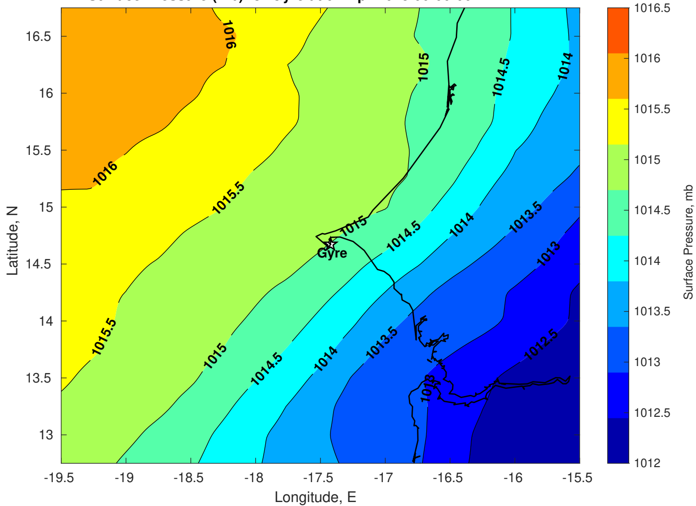
Surface Pressure (mb) for Gyre at 04-Apr-2025 00:00:00
