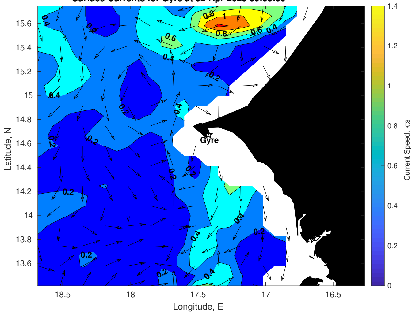
Surface Currents for Gyre at 02-Apr-2025 00:00:00
