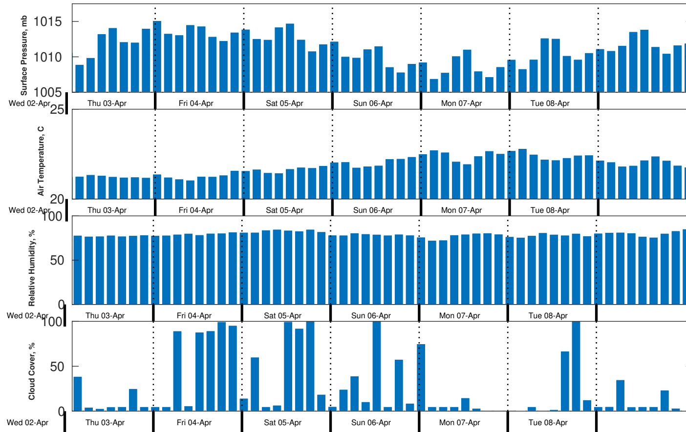
Met Forecast for Gyre from 02-Apr-2025 23:00:00 to 09-Apr-2025 23:00:00
