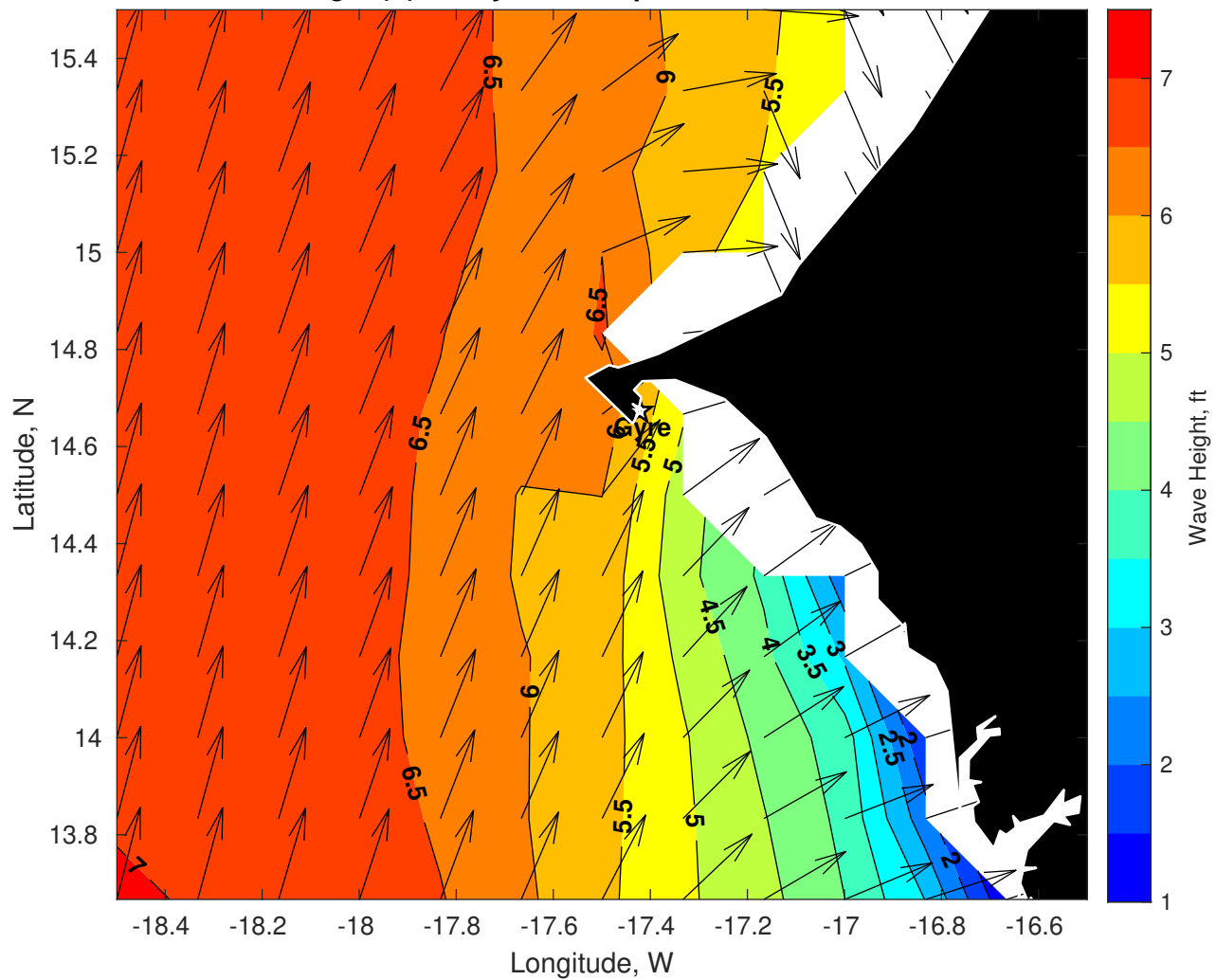
Wave Height (ft) for Gyre at 03-Apr-2025 09:00:00
