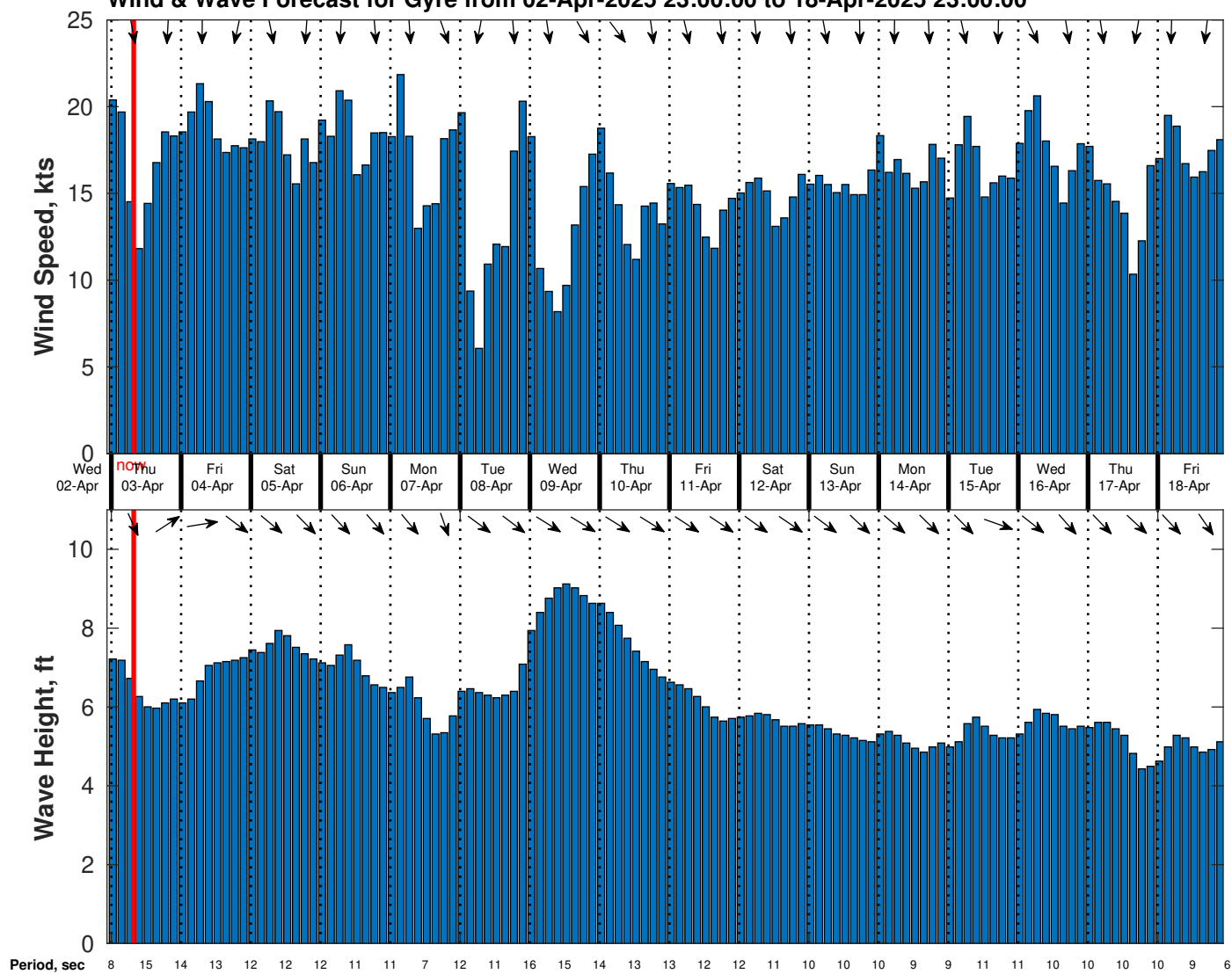
Wind & Wave Forecast for Gyre from 02-Apr-2025 23:00:00 to 18-Apr-2025 23:00:00
